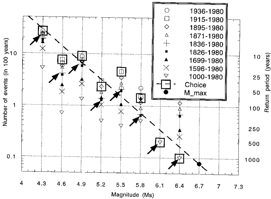
Fig. 3. Seismicity rates and maximum magnitude for SZ 4; different time periods are plotted (see legend); arrows indicate the rates suggested from the completeness analysis, large open squares indicate the selected ones. The line is the Gutenberg-Richter interpolation, on which the maximum magnitude ( M_{max} ) is evaluated.
