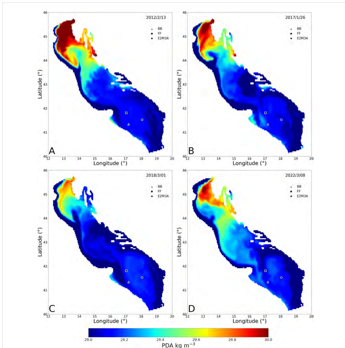
FIGURE 5 PDA map for dates when PDA is maximum in North and Middle Adriatic, for the bottom ventilation years: 2012 (A), 2017 (B), 2018 (C) and 2022 (D). We observe PDA values up to 30 kg m -3 and a tendency of the highest PDA to be located in the northernmost part of the Adriatic Sea. Due to the cyclonic circulation, dense water at the surface moves southward on the western side.
