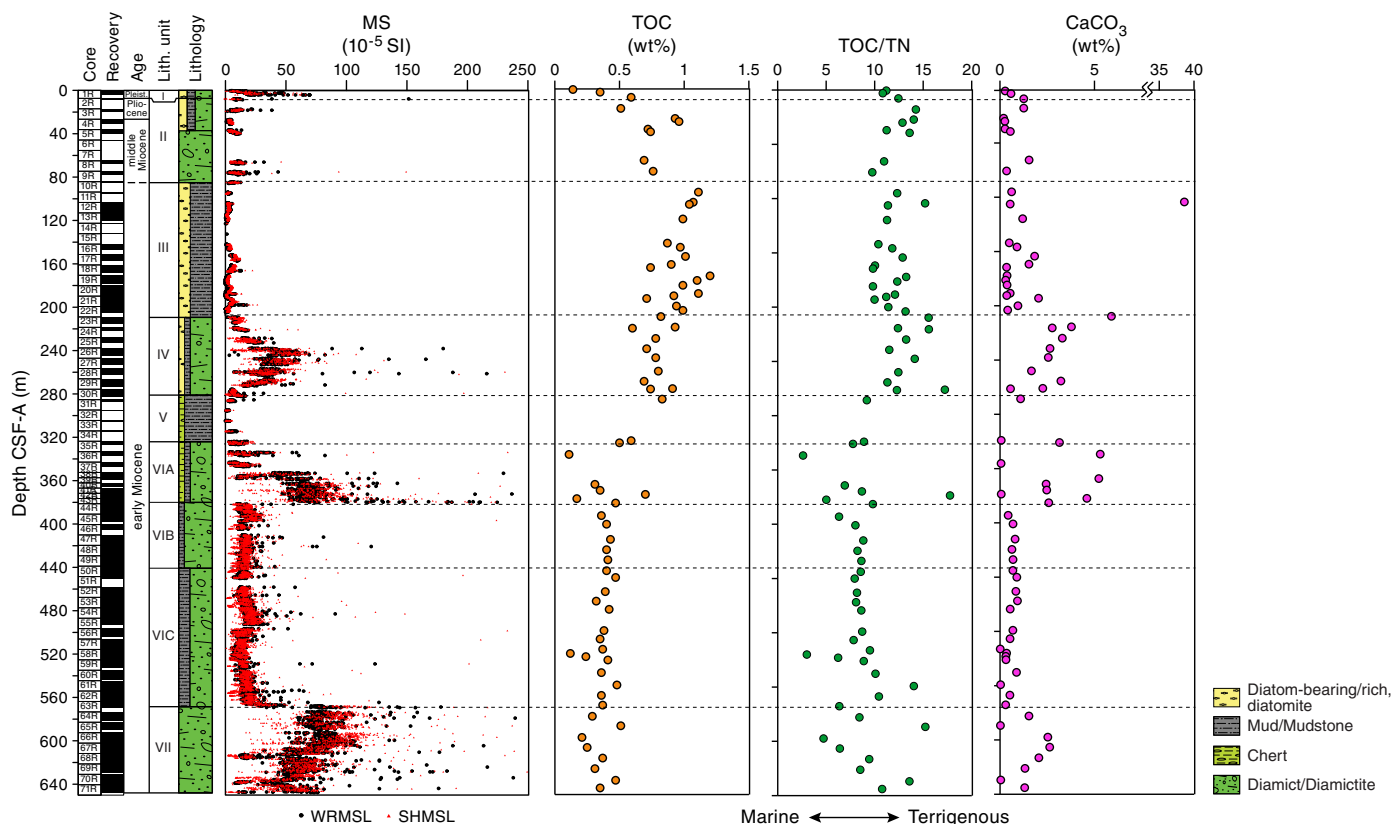
Figure F30. MS, bulk sediment TOC, TOC/TN ratio, and calcium carbonate ( \text{CaCO}_3 ), Hole U1521A. Dashed horizontal lines mark lithostratigraphic unit boundaries (see Table T2).
