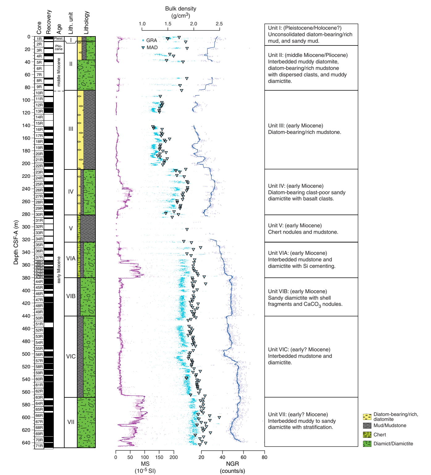
Figure F6. Lithostratigraphic summary, Hole U1521A. GRA = gamma ray attenuation, MAD = moisture and density, MS = magnetic susceptibility, NGR = natural gamma radiation.
