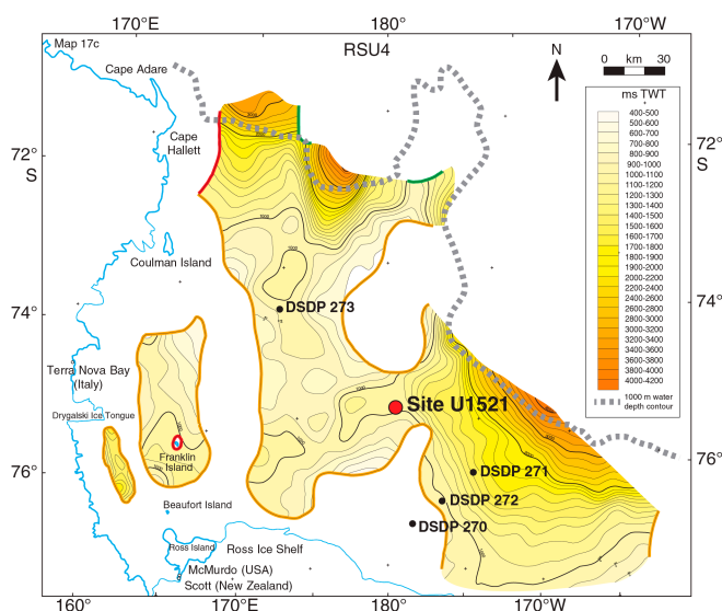
Figure F2. Depth (two-way travelttime [TWT]) contour map for regional ANTOSTRAT Ross Sea Unconformity 4 (RSU4) with location of Site U1521 and Leg 28 sites. Orange lines = erosion limits, green lines = onlap limits, red lines = intrusion limits. The modern 1000 m water depth contour, Ross Ice Shelf edge, Ross Island, and Victoria Land coast are also shown for reference. Modified from Brancolini et al. (1995). Note that the geographic orientation of this figure is inverted relative to other maps presented in the volume.
