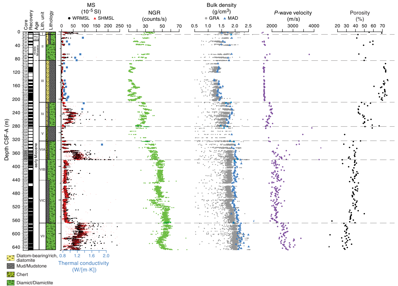
Figure F26. Physical properties summary, Hole U1521A. Dashed lines mark intervals with distinctive physical property characteristics that correlate with litho-stratigraphic units defined primarily by sedimentological characteristics (see Table T12).
