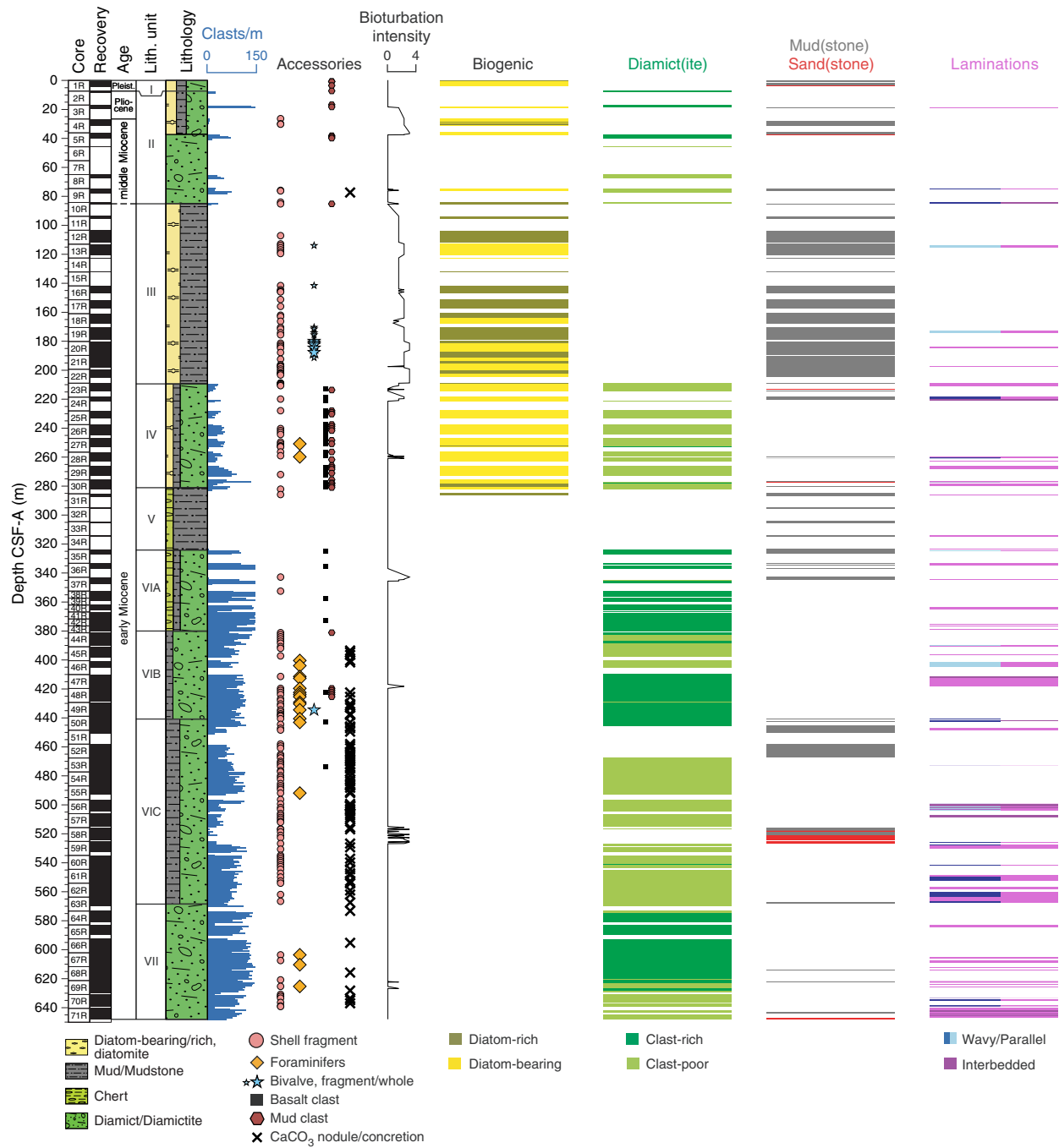
Figure F9. Lithology and sedimentary structures, Hole U1521A. Downhole profiles represent the occurrence of a described lithology or lithologic feature. Bio-turbation intensity: 0 = no apparent bioturbation (<10%) to 4 = complete bioturbation (>90%).
