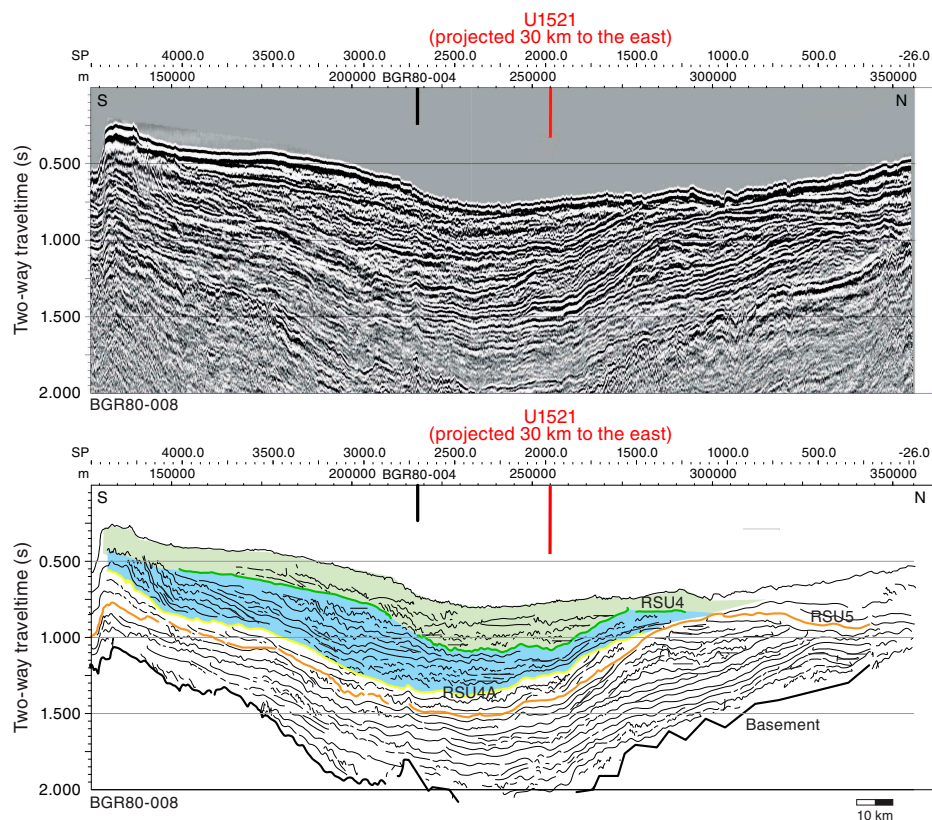
Figure F5. Top: multichannel seismic-reflection Profile BGR80-008 (green line in Figure F1). Profile was collected by BGR (Germany) in 1980 (Hinze and Block, 1984) with a 24-air gun array (23.45 L). Data were acquired with a 3000 m streamer (48 channels; first offset = 250 m, last offset = 2600 m). Bottom: interpretation of key seismic reflectors in Profile BGR80-008, showing RSU4 and other Ross Sea unconformities regionally mapped by ANTOSTRAT (Brancolini et al., 1995).
