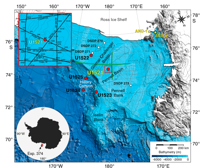
Figure F1. Bathymetric map with locations of Site U1521, other Expedition 374 sites, DSDP Leg 28 Sites 270–273, and ANDRILL Cores AND-1 and AND-2. Red box = location of inset map with Site U1521 on seismic-reflection Profile PD90-36 (Figure F3), green lines = locations of seismic-reflection Profiles BGR80-004 (east–west; Figure F4) and BGR80-008 (north–south; Figure F5). Bathymetry from Arndt et al. (2013).
