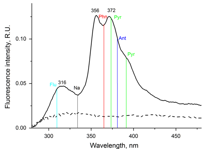
Fig. 7. Single fluorescence spectra excited at 255 nm of filtered samples collected at station M2 (continuum line) and at station M1 (dotted line). The six vertical line refer to the emission peaks of the principal components of oil. Flu: fluorene; Na: naphthalene; Phn: phenanthrene; Pyr: pyrene; Ant: anthracene.
