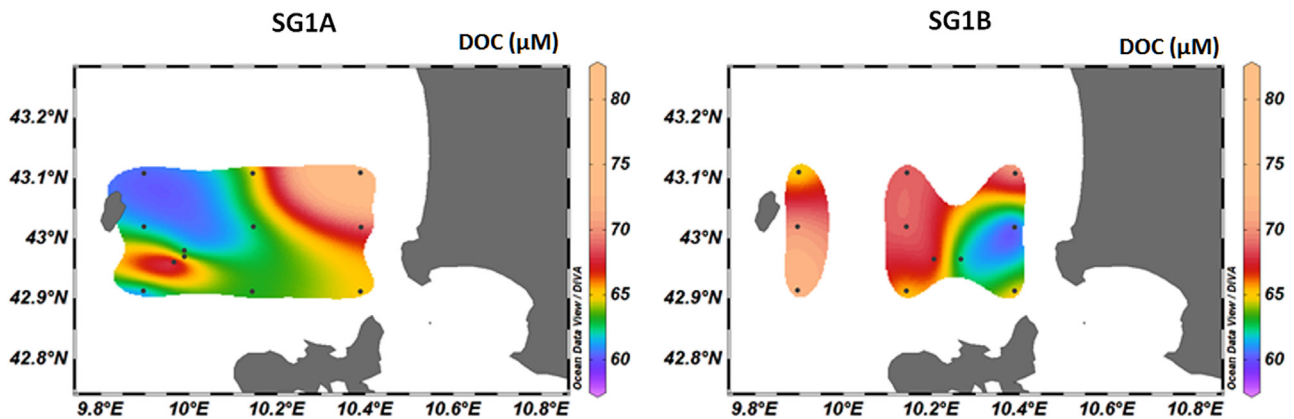
Fig. 4. Surface distribution of DOC in the two cruises. The black points refer to the data used for the interpolation.
