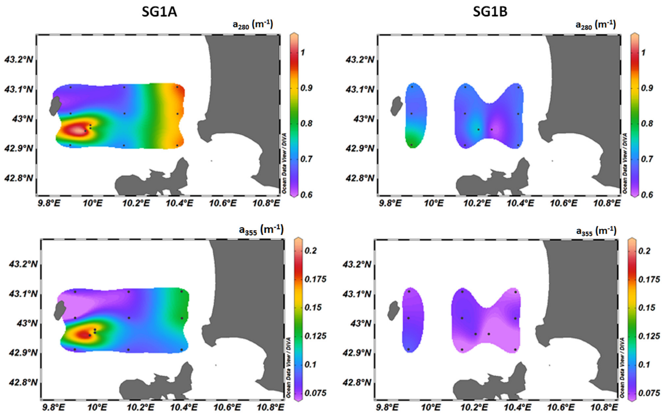
Fig. 6. Surface distribution of absorption coefficient at 280 and 355 nm. The black points refer to the data used for the interpolation.
