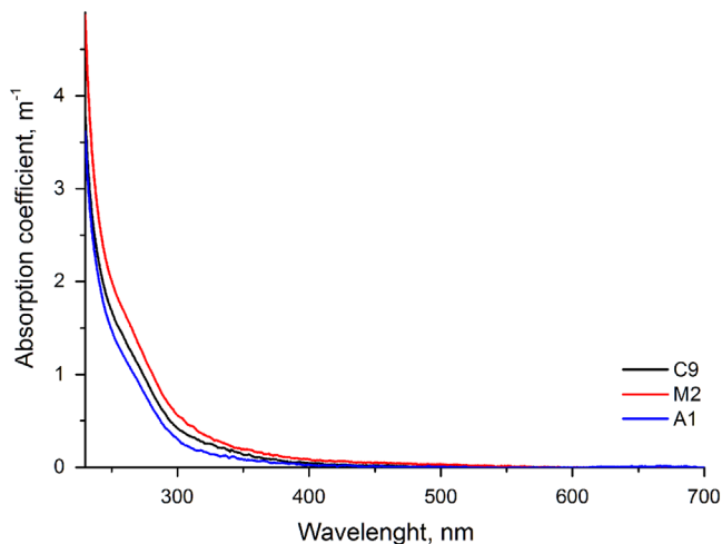
Fig. 5. Example of absorption spectra measured during SG1A at 3 stations representative of the diversity of the study area.
