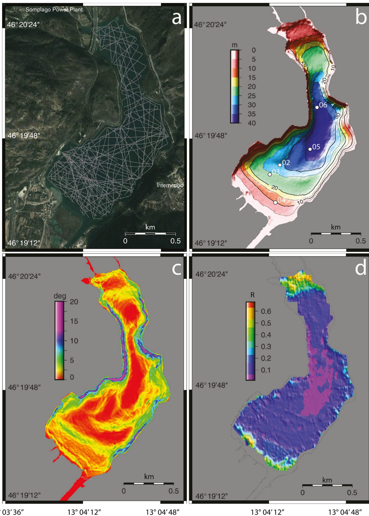
Fig. 2. Lake of Cavazzo region. a) Location map of the acquired seismic reflection data; b) bathymetric map with the location of gravity cores acquired in 2015; c) lake-floor slope; d) lake-floor reflectivity.
