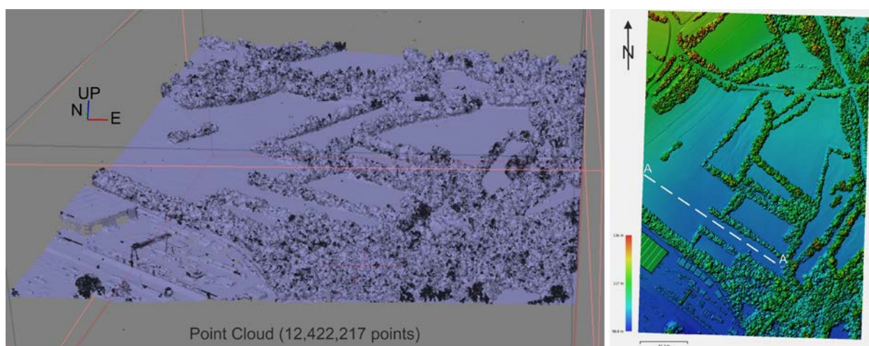
Figure 7 Left panel: Point cloud from the LiDAR dataset of Friuli Venezia Giulia. Right panel: Derived high-resolution Digital Surface Model (DSM; 20.6 cm/pixel). The elevation colour scale, ranging from 98.8 m to 136 m a.s.l., highlights subtle topographic variations along the Budoia–Aviano Thrust area.
