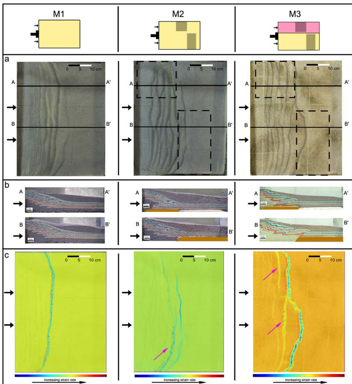
Figure 3 Main analogue models' results. a) top view at the end of the experiment; b) sections of the models at the end of the experiment (section traces visible in a), the dashed black rectangles represent the wood blocks/buried structural highs (covered by sand); c) strain rate analysis of one of the last deformation phases of the experiment. The purple arrows indicate the thrust fronts where tectonic activity is more concentrated. The pink area in M3 represents the sector with higher basal friction.
