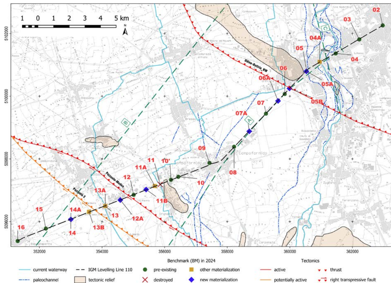
Figure 2 Planimetry of the benchmarks of the IGM levelling line 110 (measured in 2024), thrusts (from Patricelli and Poli [2020]), geological and geodynamic hints (from Marchesini et al. [2023]). RS: EPSG 6708.
