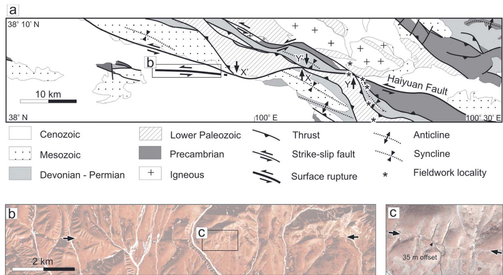
Figure 8. (a) Structure of the Haiyuan Fault at ~100°E [Geological Bureau of Qinghai Province, 1968a, 1968b]; (b) surface rupture across Quaternary sediments, located in Figure 8a; and (c) close-up of ruptures in Figure 8b. Quickbird satellite imagery from Google Earth (©2014 Google, ©2014 DigitalGlobe).
