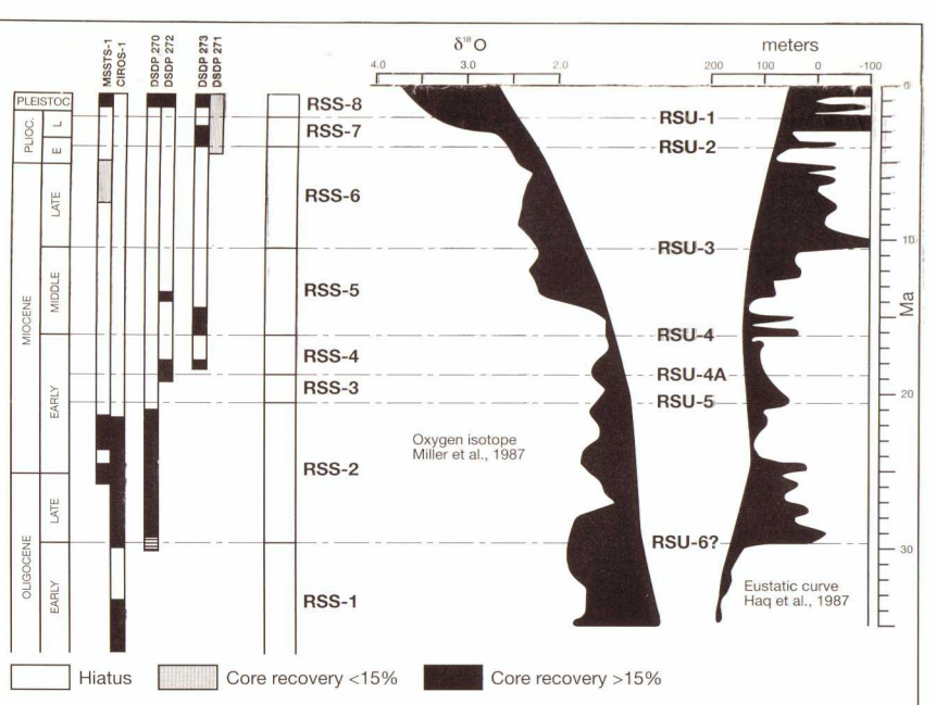
Correlation Chart of Ross Sea Seismic Sequences From Brancolini et al. [this volume]
