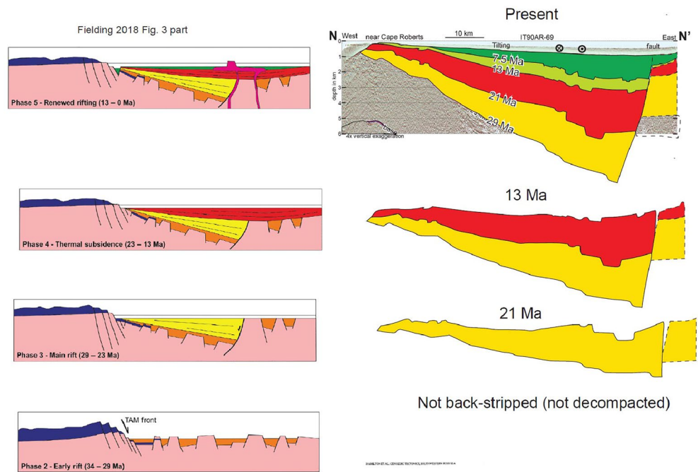
Figure 12. Comparison between the R. C. Fielding (2018) diagram on the left and our depth section, as observed in Figure 6h, on the right. The changes in sediment thickness across the fault show that there was growth on the fault and a faster vertical relief from 29 to 13 Ma than from 13 to 0 Ma (see also Figure 11).
