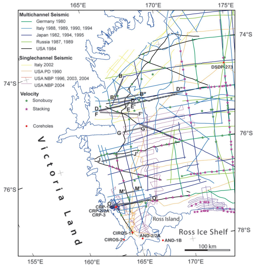
Figure 2. Location map of the seismic reflection tracklines, scientific drillholes, and depth-time charts derived from sonobuoys (green stars) or the interval velocities derived from stacking velocities (magenta stars). The seismic profiles shown in the following figures are denoted as B-B'' through O-O'. The densely distributed depth-time velocity charts and thus the 3D velocity model and depth conversion cover this map and greater than 200 km to the east of this figure.
