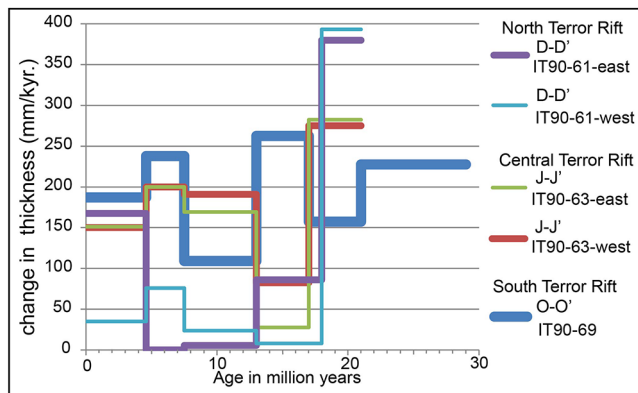
Figure 11. Measurements of sediment thickness changes over time in the Terror Rift. These measurements were made along the O-O' profile in the southern Terror Rift and are related to the western flank, along profile J-J' in the central Terror Rift, and along profile D-D', in the northern Terror Rift, which are both related to the eastern and western rift flanks (see Figures 6b–6h for measurement location). The sediment thickness changes are high between 29 and 13 Ma in the south and are smaller between 17 and 13 Ma in the central Terror Rift and after 18 Ma in the north.
