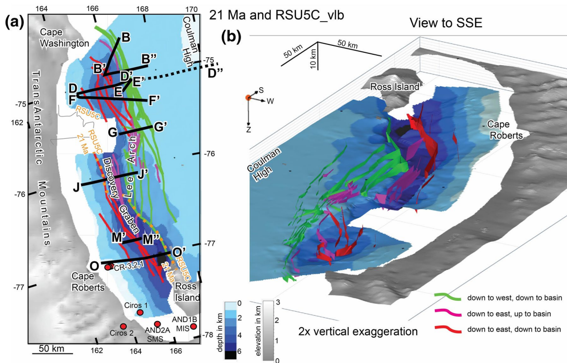
Figure 5. Plan (a) and oblique (b) views of the merged 21 Ma (west) and RSU5C_vlb (east) unconformities. The orange dashed line on the plan map (a), which mostly runs along two of the large faults, shows the limit of the merged unconformities. RSU5C_vlb and 21 Ma were correlated across the boundary as the same unconformity near the label "Graben." We acknowledge that this correlation has certain limitations, including interpretation of the vertical component across faults. These horizons and the faults are all displayed in depth with two times vertical exaggeration. The northern rift trends N-S, while the southern rift trends NNW-SSE. A large fault(s) may be present west of these grids along the front of the Transantarctic Mountains. The faults colors indicate the sense of vertical motion (red color = eastward and green color = westward).
