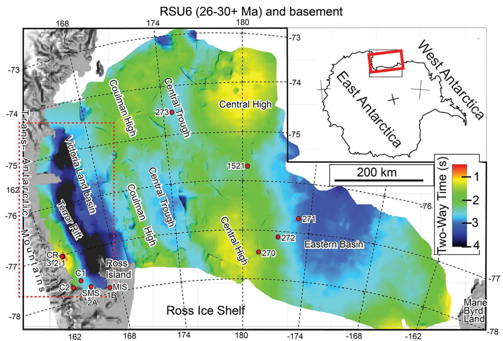
Figure 4. Ross Sea basins that are evident on the mid-Cenozoic RSU6 horizon. This horizon is deeper than 4 s two-way time in part of the Terror Rift. The scientific core holes are labeled with red dots: 270, 271, 272, and 273 are Deep Sea Drilling Project; CRP 3-2-1 are Cape Roberts Project; C1 and C2 are Ciro 1–2; MIS-1B and SMS-2A are Andrill and U1521 is IODP. The red dashed rectangle indicates the volume of Figure 5.
