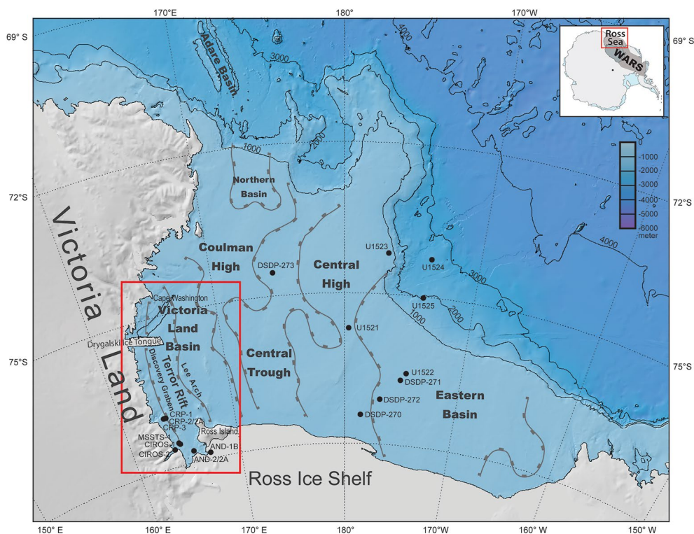
Figure 1. Ross Sea bathymetric map with the main structural highs and basins outlined in gray and the drillhole positions shown (contours every 1,000 m). The red box in the inset map displays the location of this figure, and the red rectangle in the figure locates the study area of the Terror Rift in the western Ross Sea, as observed in Figures 2 and 5. The inset map shows the location of the West Antarctic Rift System (WARS). The DEM model was constructed with GeoMapApp ( www.geomapapp.org ; CC by Ryan et al., 2009).
