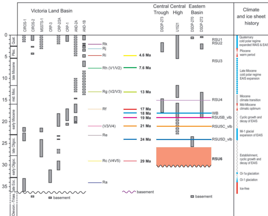
Figure 3. Time-distribution of the well stratigraphy and regional seismic reflectors/unconformities for the Ross Sea. Stratigraphy of the wells CIROS-1 (Barrett, 1986, 1989; Harwood, 1989; Sagnotti et al., 1998; G. S. Wilson et al., 1998) and CIROS-2 (Barrett and Scientific Staff, 1985; Winter & Harwood, 1997). CRP-1, CRP2/2A, and CRP-3 (Cape Roberts Science Team, 1998, 1999, 2000); AND-1B and AND2/2A (SMS Science Team, 2010); DSDP 270, 272, 273 (Hayes & Frakes, 1975; Savage & Ciesielsky, 1983) with updating of the DSPD 270 after Kulhanek et al. (2019). Seismic reflectors/unconformities interpreted in the Victoria Land Basin: Ra to Rk unconformities from Fielding et al. (2008); V1 to V5 from Cooper et al. (1987a); ANTOSTRAT Unconformities (RSU) RSU1 to RSU6 from Brancolini et al. (1995a, 1995b); Wb reflector at the bottom of DSDP 273 from Savage and Ciesielsky (1983), Sauli et al. (2014); RSU5B_vlb and RSU5C_vlb from this work and Brancolini et al. (1995a, 1995b); RSU5D_vlb from this work and C. Sorlien et al. (2019), Brazell, (2017); Reflectors 29, 21, and 17 Ma from Hamilton et al. (2001), R. C. Fielding (2018) (reflector 21 Ma also from Fielding and Thompson, 1999). Climate and ice sheet history from R. C. Fielding (2018). Time scale from the International Chronostratigraphic Chart 2019/05 ( www.stratigraphy.org ; Cohen et al., 2013). See Figures 1, 2 and 5 for drillhole locations.
