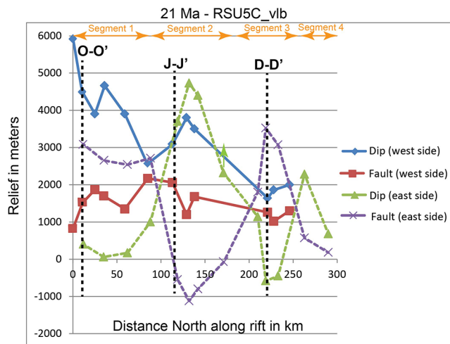
Figure 10. Components of Terror Rift relief due to faulting and due to dip for the eastern margin (dashed) and western margin (solid). The positive dip on the eastern side is to the west, while the positive dip on the western side is to the east. The eastern margin has four segments, where the relief alternates between faulting and dip. The western margin relief is due to both faulting and to dip, except in the south, where it is mostly due to dip. Relief on the western margin does not include any proposed fault system between the Transantarctic Mountains and the Ross Sea.
