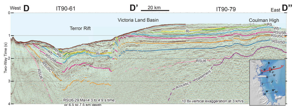
Figure 8. Composite multichannel seismic reflection profile across Terror Rift, Victoria Land Basin and Coulman High, displayed in two-way time and located in Figures 2 and 5. The part of this profile between D and D' is displayed in depth with less vertical exaggeration in Figure 6b. The entire profile images the Terror Rift (TR) within the older Victoria Land basin (VLB). There has been little deformation east of the Terror Rift since RSU6 (26–30+ Ma), and even less after RSU5D_vlb (24 Ma), even while the Terror Rift experienced two to 3 km of relative vertical motion here.
