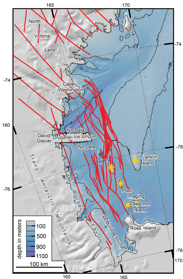
Figure 7. Map view of the interpreted faults. Faults are shown in red: onshore from Rosetti et al. 2006 and offshore from our mapping, except for the Transantarctic Mountains frontal fault system from Olivetti et al. (2018). The sea floor is displayed in shades of blue, and the main volcanic features are marked on the eastern Terror Rift flank with stars.
