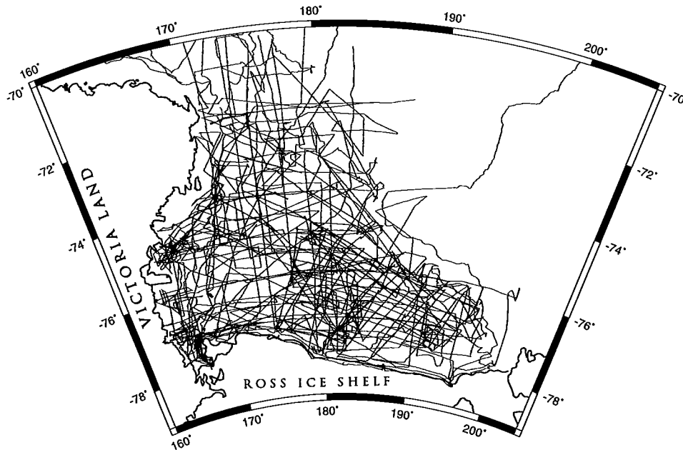
Fig. 3. Trackline map for Ross Sea cruises that collected bathymetry data used to make the bathymetric map shown in Atlas Plate 1.
