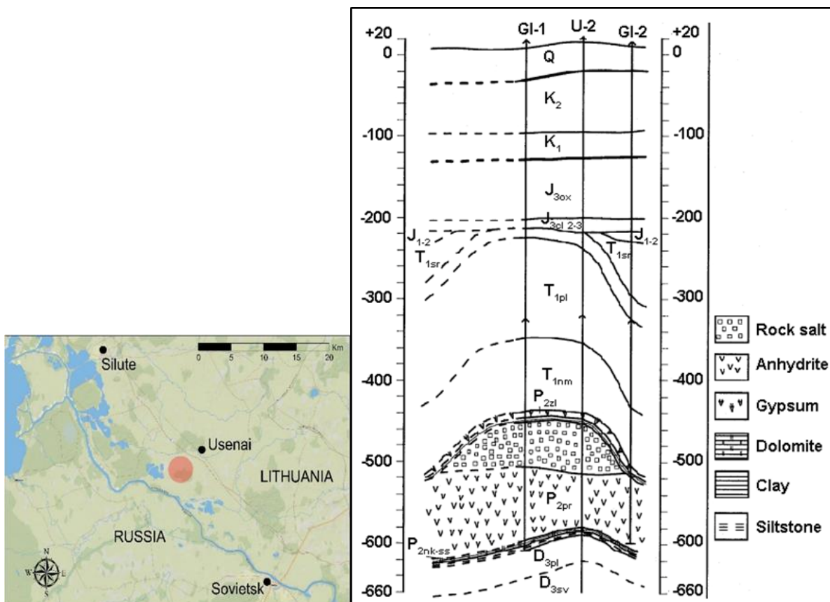
Figure 52: a) Location of the salt dome in the Usėnai area, b) Geological cross section across Usėnai salt dome. Q-Quaternary, K2-Upper Cretaceous; K1-Lower Cretaceous, J3ox- Oxfordian Upper Jurassic, J3cl- Callovian Upper Jurassic; J1-2-Lower-Middle Jurassic, T1sr- Šarkuvos Fm. Lower Triassic, T1tr- Tauragės Fm. Lower Triassic, T1pl- Palangos Fm. Lower Triassic, T1nm- Nemuno Fm. Lower Triassic, P2pr-Prėgliaus Fm. Upper Permian Series (Lopingian), D3pl- Pļavinas Fm. Upper Devonian; D3sv- Šventosios Fm. Upper Devonian.
