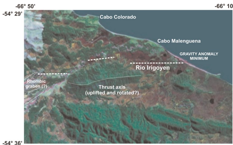
FIGURE 3 | SPOT image of the eastern termination of the Río Irigoyen valley. Here the underlapping segments of the Magallanes-Fagnano fault system are arranged in an-echelon geometry. The location of the gravity minimum along the coast, and centered in correspondence of the Río Irigoyen estuary, is also indicated.
