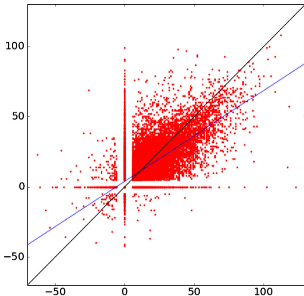
Figure 2.3.2. BLT comparisons between ARMOR3D weekly (product 2.3.1) and in situ: scatterplot diagram between Argo profiles in situ BLT in the Tropical Pacific (15°N-15°S,130°E-80°W) (abscissa), and the corresponding collocated BLT from ARMOR3D (ordinate); units are metres. The black line along the diagonal corresponds to the perfect fit; the flatter blue line corresponds to the linear regression between ARMOR3D and in situ data.
