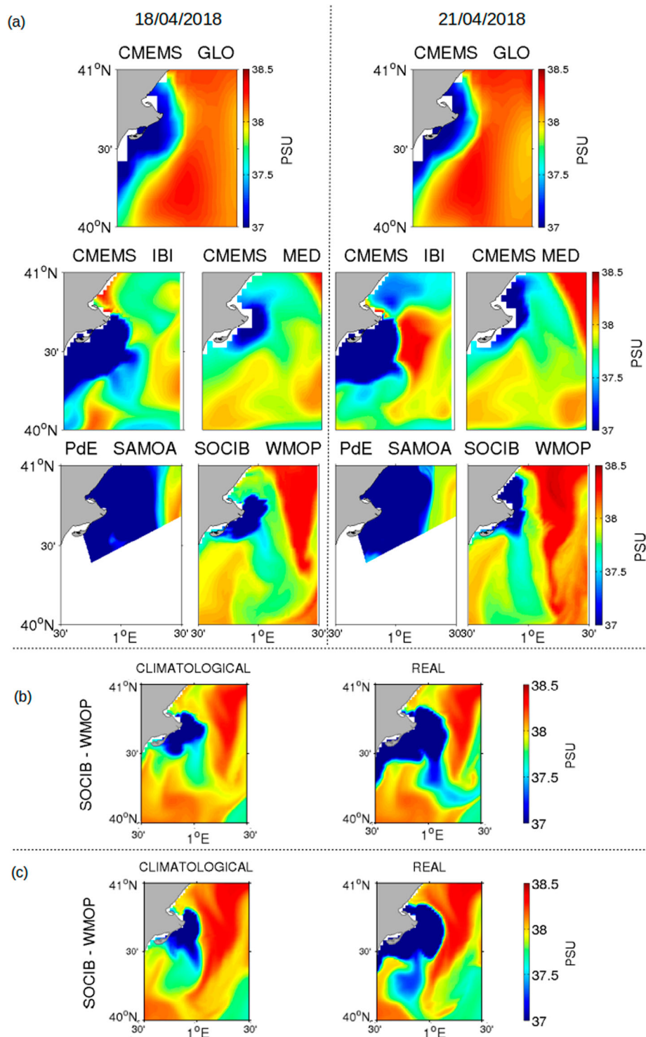
Figure 4.10.3. (a) Maps of surface salinity distribution in the Ebro River Delta from 5 different ocean models: (i) CMEMS GLO-MFC (Product ref. 4.10.3); (ii) CMEMS IBI-MFC (Product ref. 4.10.4); (iii) CMEMS MED-MFC (Product ref. 4.10.5); (iv) PdE-SAMOA (Product ref. 4.10.12); (v) SOCIB-WMOP (Product ref. 4.10.9). Panel (a) is divided in 18 and 21 April 2018, respectively. (b) 18-April-2018 WMOP (Product ref. 4.10.9) daily average surface salinity distribution and currents (hindcast simulation climatological and real runoff) and (c) 21-April-2018 WMOP (Product ref. 4.10.9) daily average surface salinity distribution and currents (hindcast simulation climatological and real runoff).
