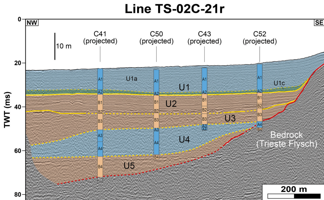
Fig. 8. The TS-02C-21r high-resolution seismic profile (see Fig. 1 for location and Fig. 4 for symbols and abbreviations). Seismic units and their environmental interpretation (based on recognized features as well as on correlation between cores and the present profile) are shown.
