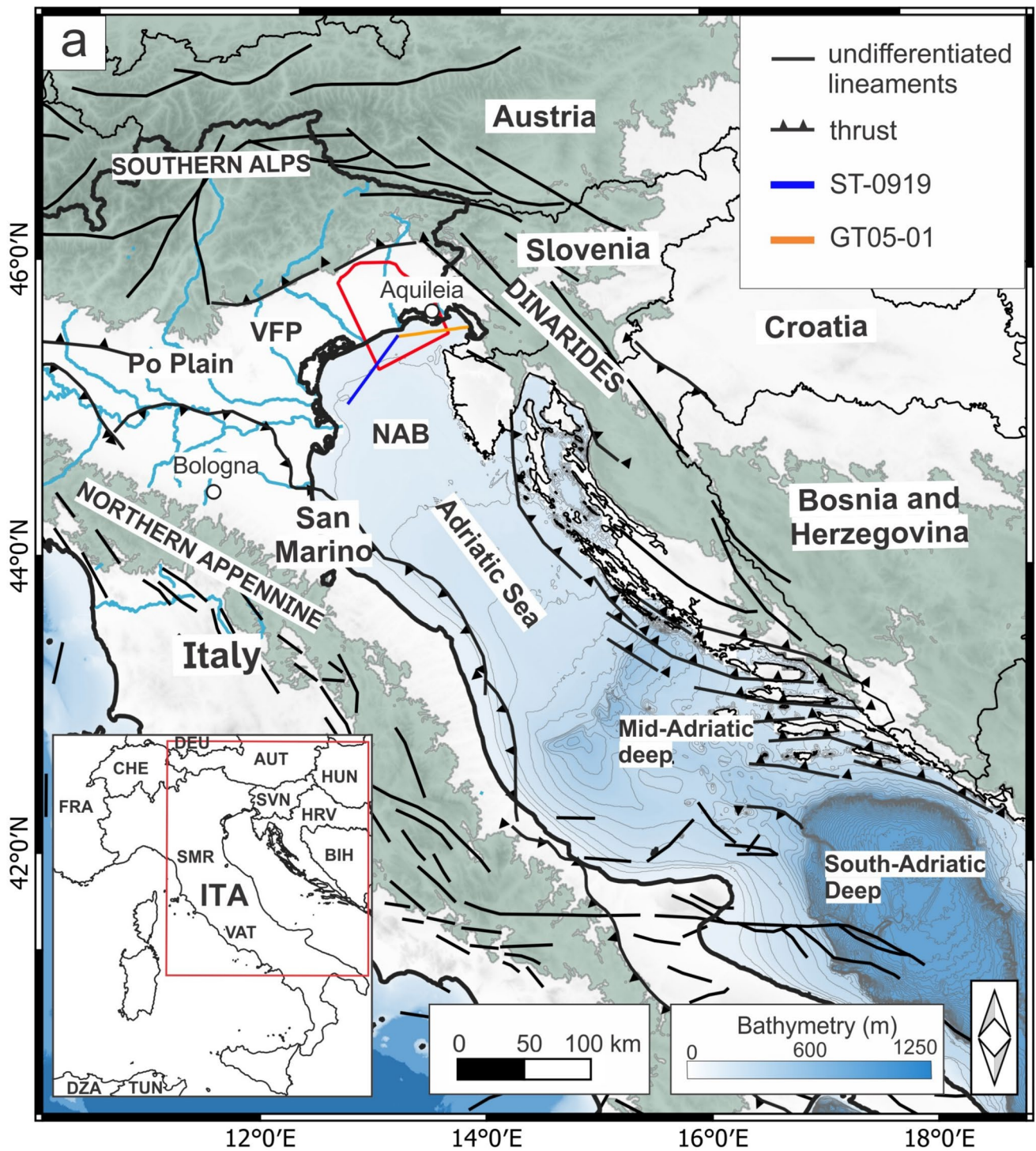
Fig. 1 (a) Simplified structural geology map of the Adriatic Basin and surrounding landmasses. The study area ( solid red line ) is surrounded by External Dinarides to the east and Southern Alps to the north. Tectonic lineaments, including major undifferentiated faults and thrusts in Italy and surrounding regions are modified after Palano (2015). Seismic lines ST09-19 and GT05-01 are sourced from Zec-
