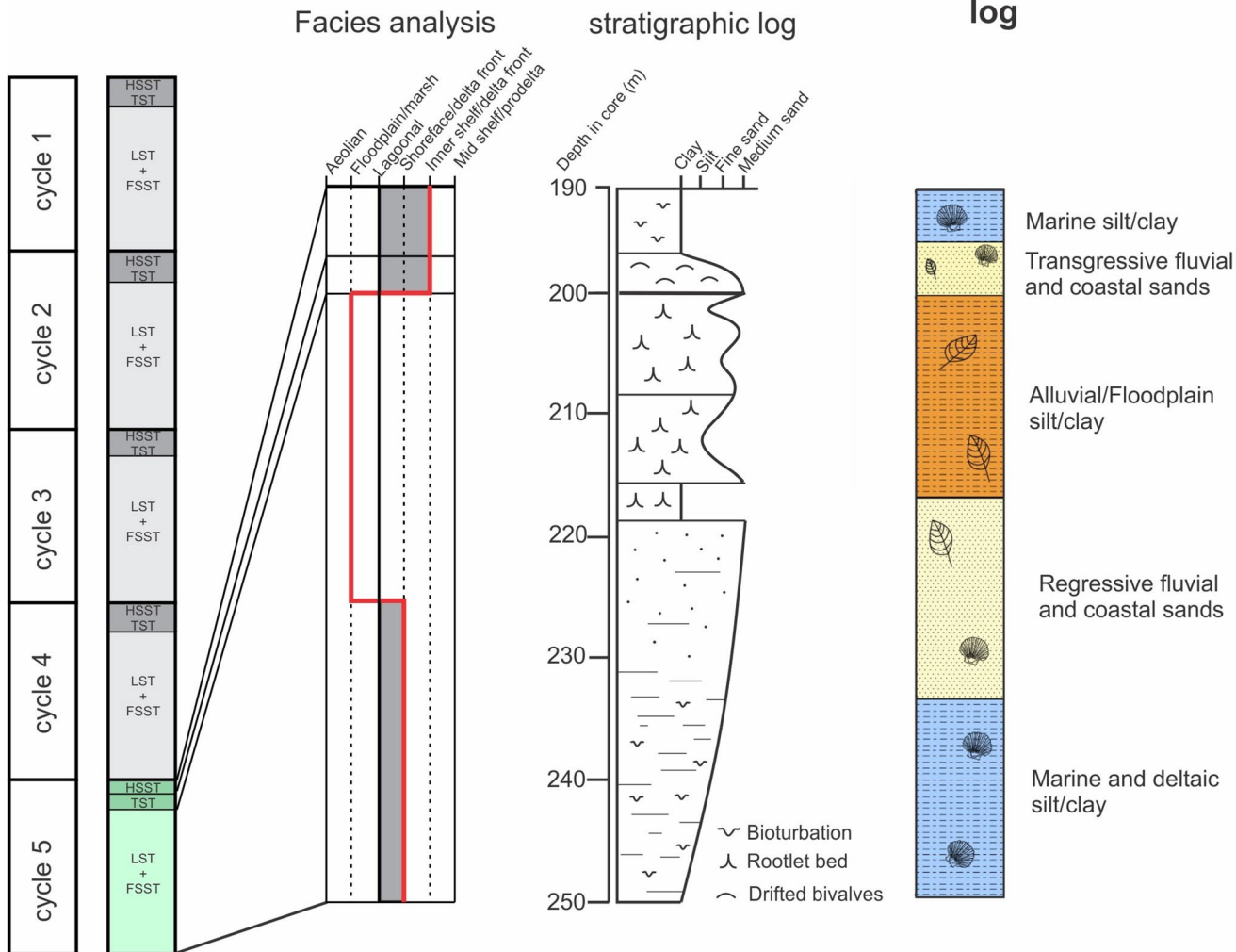
Fig. 3 Conceptual representation of a pseudo-stratigraphic log. (left) a conceptual borehole exhibits five successive R-T cycles with constant thickness, each composed of a regressive phase (FSST+LST) and a transgressive phase (TST+HST). Thickness proportions are derived from the 5th cycle recorded in Venezia 1 (Amadori et al. 2020), whereas the regressive phase constitutes 85% of the cycle
