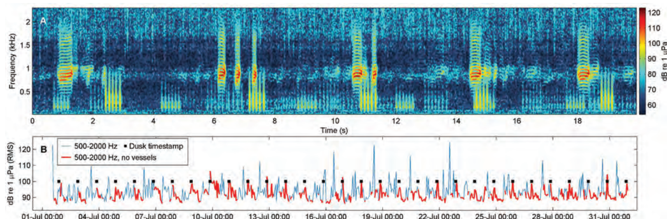
Fig. 3: A) Segment of a typical fish chorus, recorded during the night of 04-07-2022, 22:22 local time ( N_{FFT} = 4096 samples, Hamming window, 90% overlap). B) Time series of ambient noise levels (RMS) at the 500–2000 Hz frequency band during July 2022. The black squares mark dusk time per day and were arbitrarily plotted at y = 100 dB.
