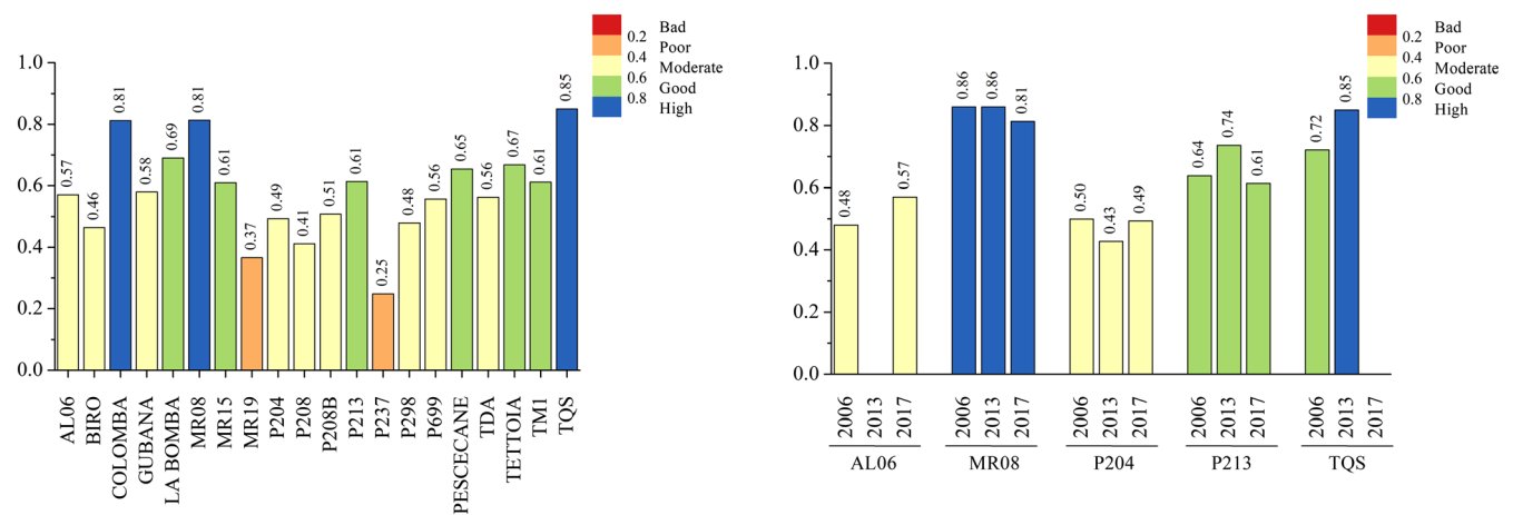
FIGURE 7 Values of the NAMBER index for multiple years (2006, 2013, and 2017) in a subset of biogenic reefs investigated off Chioggia (AL06, MR08, P204, P213, and TQS). Colour scale indicate the ecological status classes.
