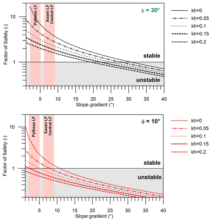
Fig. 12. Factor of safety calculations based on the pseudostatic approach (FOSPS) for seismic coefficients k_h from 0 to 0.2. Top: scenario of sediments with a friction angle of 30^\circ . Bottom: scenario of sediments with a friction angle of 10^\circ . Instability may be attained for the Xauen and Central Landslide Fields (LF) if k_h > 0.05 , and for the Pytheas LF k_h > 0.1 . \phi friction angle; k_h pseudostatic seismic coefficient.
