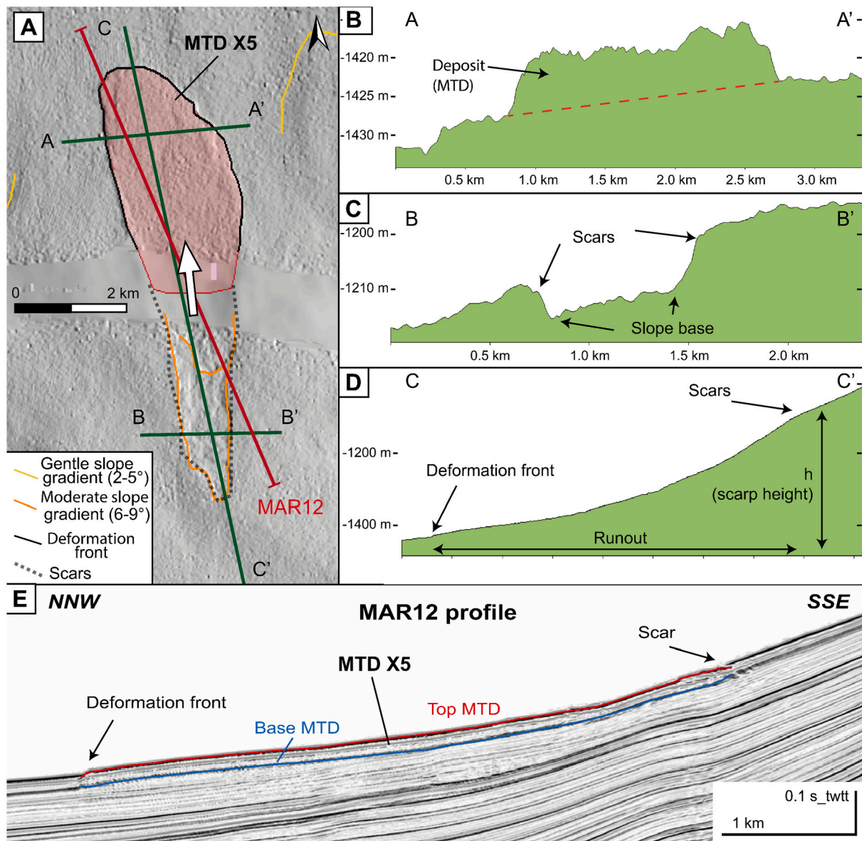
Fig. 5. Characterization of a submarine landslide using bathymetry (A), slope profiles (B, C, D) and seismic reflection profile (E): example of MTD X5 along the Xauen Bank northern flank. The white arrow indicates direction of transport of the submarine landslide.
