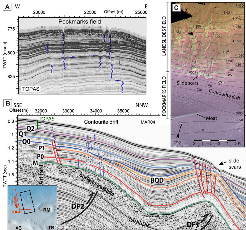
Fig. 10. Fluid escape and compactional fault features through contourite drift in the SAR region (north Xauen Bank). A. Sub-seabed expression of fluid escapes and pockmarks on ultra-high resolution seismic reflection data (TOPAS). Location in B. B. High-resolution seismic reflection data showing the deformation below the contourite drift, associated to faults and fluid escapes. The normal faults here are interpreted as due to fold extrados extension from blind thrusts. Inset: in red location of MAR04 and TOPAS profiles, black rectangle corresponds to bathymetric zoom in C. C. Seabed expression of pockmarks and landslide scar. Bathymetric data with contours every 50 m. XB, Xauen Bank; TB, Tofino Bank; RM, Ramon Margalef Seamount. (For interpretation of the references to colour in this figure legend, the reader is referred to the web version of this article.)
