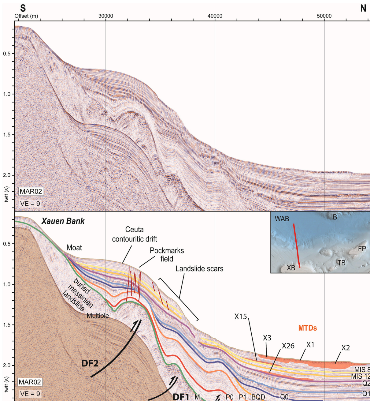
Fig. 6. High-resolution profile from Marlboro 1 campaign (MAR02), between the Xauen Bank (XB) and the southern WAB. It shows localization of landslide scars along slopes north to the Xauen Bank, where slope gradient is affected by contouritic sedimentation (Ceuta contourite drift) and northward vergence thrusts (DF1, DF2) as well as mass transport deposits (Xx mapped in Fig. 2B). TB Tofiño Bank, FP Francesc Pagès Seamount, IB Ibn Batouta seamount. P0, P1, BQD, Q0, Q1, Q2, MIS12 and MIS8 refer to seismic reflectors defined in Fig. 4.
