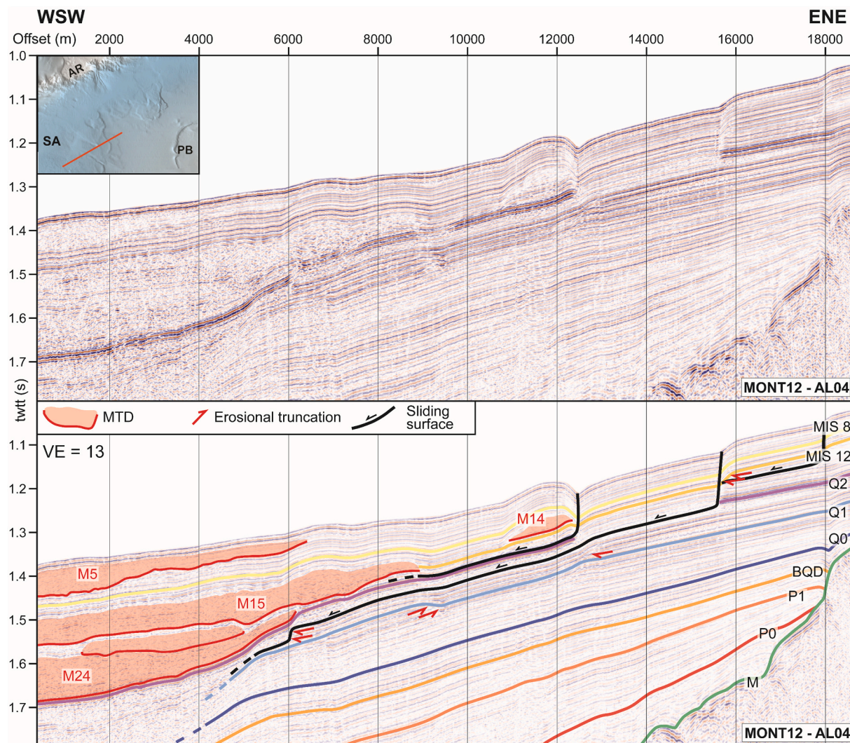
Fig. 7. High-resolution profile from MONTERA campaign (AL04), in the southern SAB. It highlights buried MTDs downward the slope and three decollement levels above the Q1 reflector. Mx Mass transport deposits represented in map Fig. 2B. AR Alboran Ridge, PB Pytheas Bank, M, P0, P1, BQD, Q0, xx refer to seismic reflectors defined in Fig. 4.
