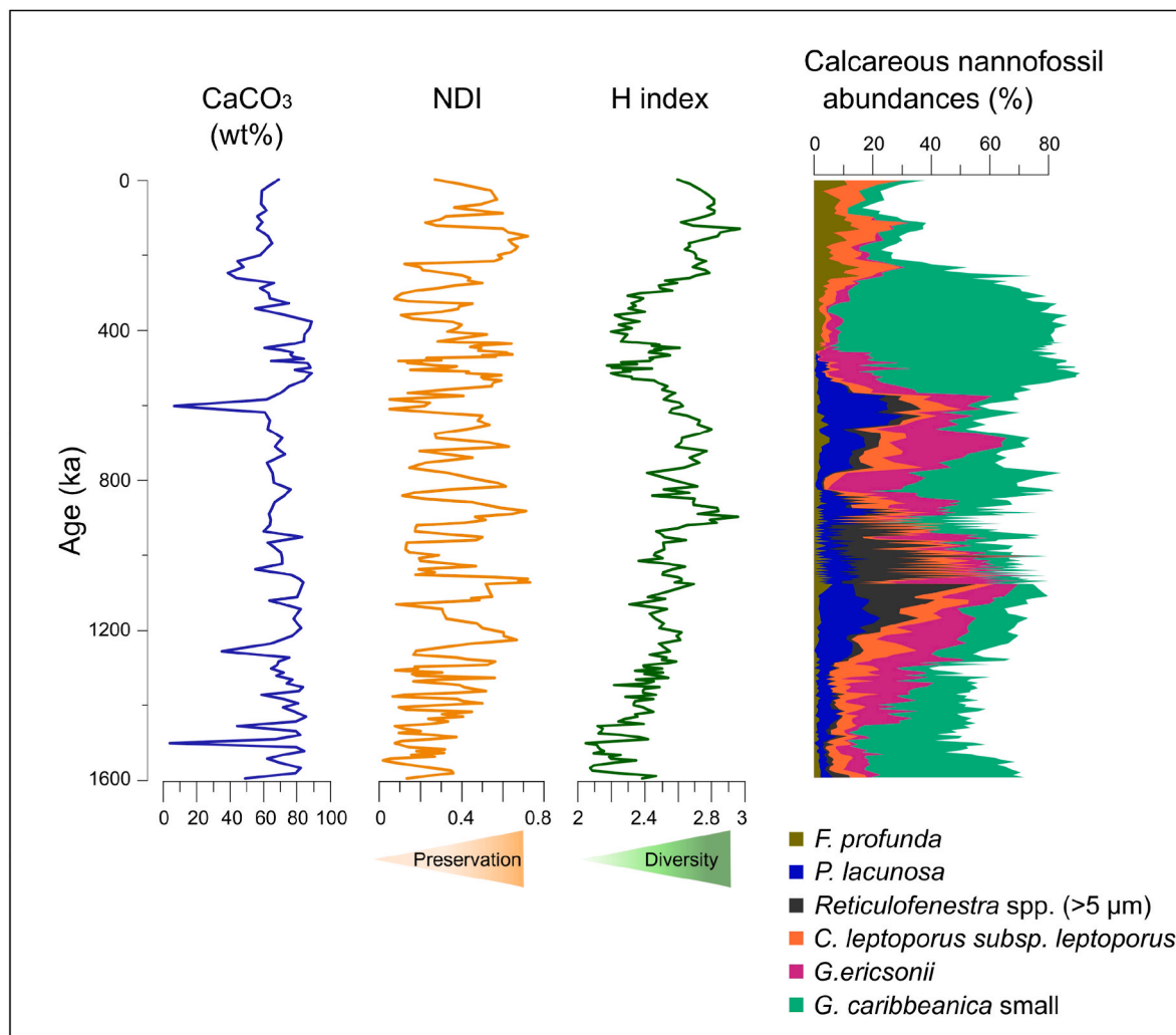
Fig. 3. Previously published data from Site 1209 plotted against age (ka): CaCO 3 (wt%) measured on bulk sediment (Lupi et al., 2012; Bordiga et al., 2013); Nannofossil Dissolution Index (NDI; Bordiga et al., 2013); H index (Lupi et al., 2012); relative abundances (%) of the selected species within the calcareous nannofossil assemblages (Bordiga et al., 2014; Lupi et al., 2012, 2019; newly collected data).
