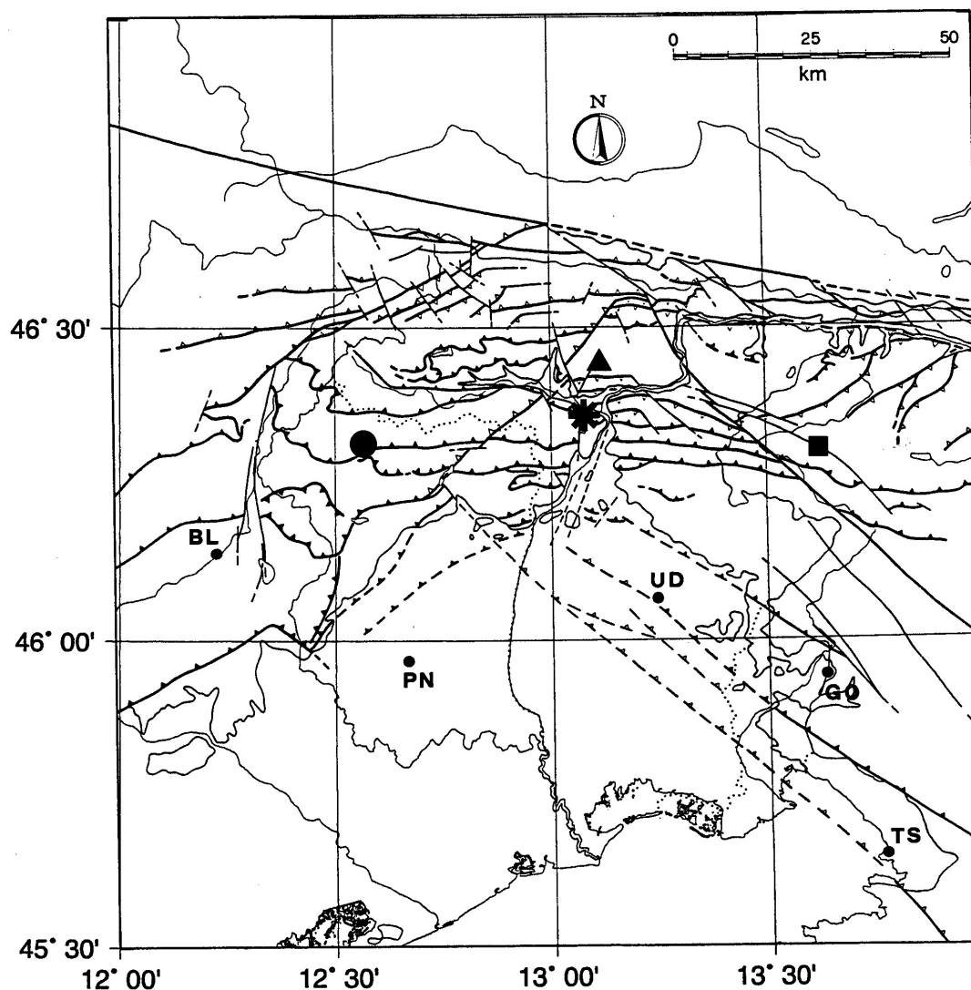
Fig. 1 - Schematic tectonic map of the north-eastern Italy and western Slovenia; line and dashed line: subvertical fault, toothed line: thrust. The location of the moderate-size earthquakes considered in the present study are marked with different symbols; full circle: 1996 Claut mainshock, full triangle: 2002 Sernio mainshock, asterisk: 1988 Mena mainshock, full square: 1998 and 2004 Bovec mainshocks. BL: Belluno town; PN: Pordenone town; UD: Udine town; GO: Gorizia town; TS: Trieste town. Longitude-degrees (horizontal axis), latitude-degrees (vertical axis). Friuli-Venezia Giulia map with the epicenters of the earthquakes analyzed.
