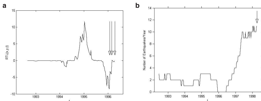
Fig. 4 - Temporal variation of the RTL parameter calculated in the epicenter of the M_D 4.3 Claut earthquake (a). Number of earthquakes per year (b). The times of the occurrence of the two main foreshocks, with M_D 3.5 and M_D 3.8 and of the tested earthquake are marked with an arrow.
