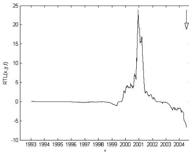
Fig. 8 - Temporal variation of the RTL parameter for the M_D 5.1 Bovec04 earthquake with 2t_0 equal to 19 months. The time of the occurrence of the tested earthquakes is marked with an arrow.
