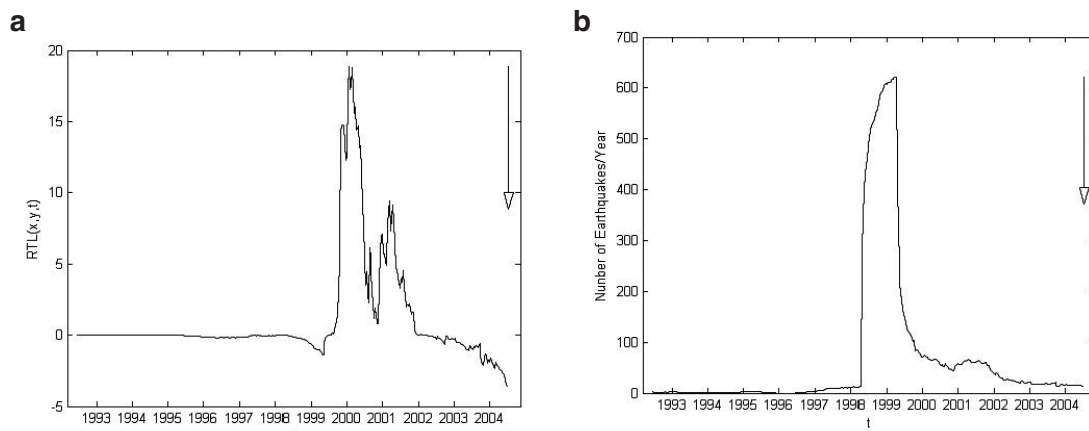
Fig. 7 - Temporal variation of the RTL parameter calculated in the epicenter of the M_D 5.1 Bovec04 earthquake (a). Number of earthquakes per year (b). The time of the occurrence of the tested earthquake is marked with an arrow.
