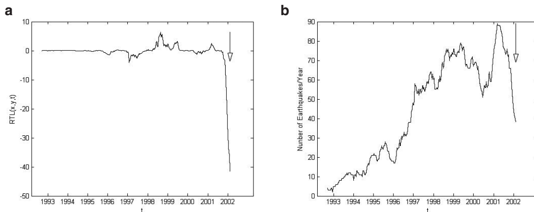
Fig. 6 - Temporal variation of the RTL parameter calculated in the epicenter of the M_D 4.9 Sernio earthquake (a). Number of earthquakes per year (b). The time of the occurrence of the tested earthquake is marked with an arrow.
