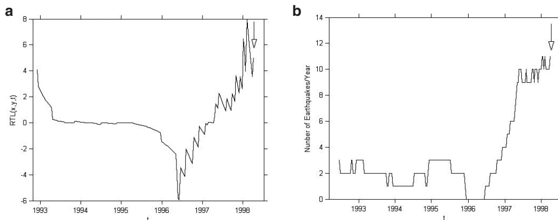
Fig. 5 - Temporal variation of the RTL parameter calculated in the epicenter of the M_D 5.6 Bovec98 earthquake (a). Number of earthquakes per year (b). The time of the occurrence of the tested earthquake is marked with an arrow.
