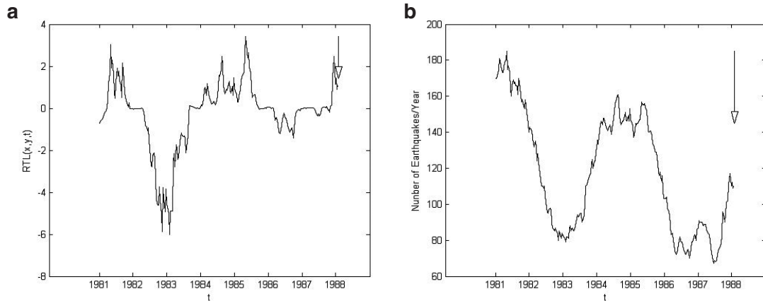
Fig. 3 - Temporal variation of the RTL parameter calculated in the epicenter of the M_D 4.1 Mena earthquake (a). Number of earthquakes per year (b). The time of the occurrence of the tested earthquake is marked with an arrow.
