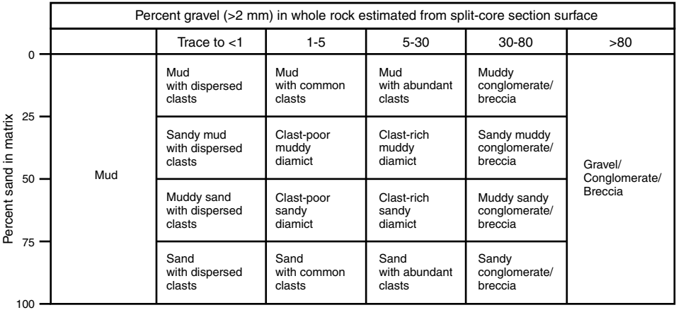
Figure F9. Classification scheme for sediments that contain mixtures of pelagic biogenic and siliciclastic components, Expedition 374.
