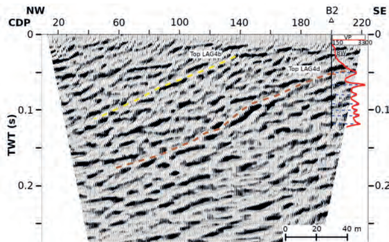
Fig. 6 - Post-stack migrated section of line 1 P with superimposed the P time-converted velocity from VSP data (red line). BW: base of weathering. The Top LAG 4d and Top LAG 4b horizons were interpreted as the tops of the respective lithofacies characterising the Campotosto Member of the Laga Flysch Formation.
