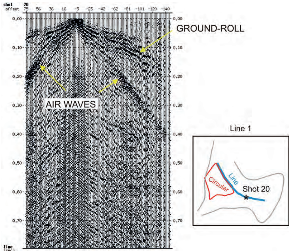
Fig. 10 - Common shot gather of line 1 P.
