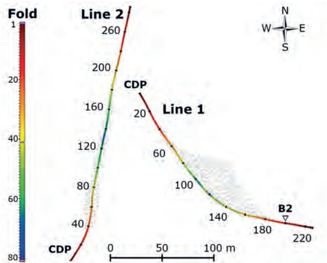
Fig. 5 - Calculation of CDPs and their coverage for lines 1 and 2, demonstrating that many points (grey dots) lie outside the line (especially for line 1). The maximum coverage in the central zone of the lines was approximately 80 traces per CDP.
