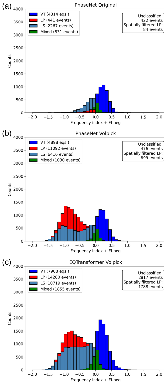
Figure 7. Histograms of labeled events according to frequency index (FI) + FI-neg from (a) PhaseNet Original, (b) PhaseNet Volpick, and (c) EQTransformer Volpick. Numbers of unclassified and spatially filtered LP events are shown in the boxes in the right corner of each plot. The color version of this figure is available only in the electronic edition.
