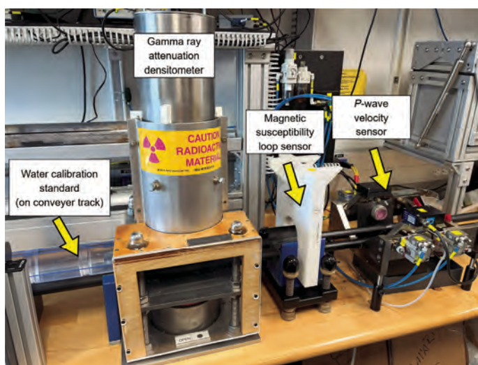
Figure F16. WRMSL, Expedition 403. Water standard shown was measured at the end of each core for QA/QC purposes.
