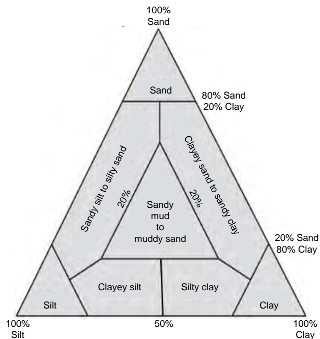
Figure F8. Ternary diagram for terrigenous clastic sediments composed of >70% siliciclastic material without gravel, pebble, or cobble (after Shephard, 1954), Expedition 403.
