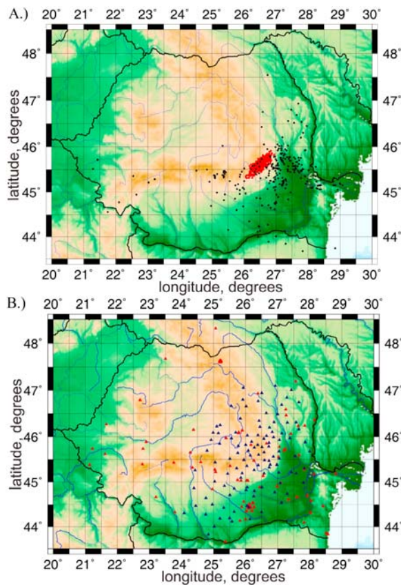
Figure 3. Data used in this study. (a) Earthquake distribution. Red and black dots show intermediate-depth and crustal events, respectively. (b) Seismic stations: blue for temporary network from CALIXTO and red for stations which are sending data to RO-NDC.
