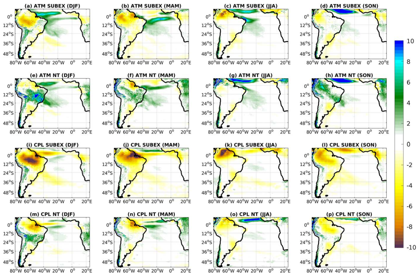
Figure 8. Precipitation bias (in \text{mm d}^{-1} ) over the South Atlantic domain with respect to observations (GPCP). (a–d) Standalone atmospheric model (ATM) using SUBEX scheme; (e–h) ATM model using NT; (i–l) coupled model (CPL) using SUBEX, and (m–p) CPL with the NT scheme. Biases are computed over the period 1988–1997 of austral summer (DJF, left), autumn (MAM, center left), winter (JJA, center right), and spring (SON, right).
