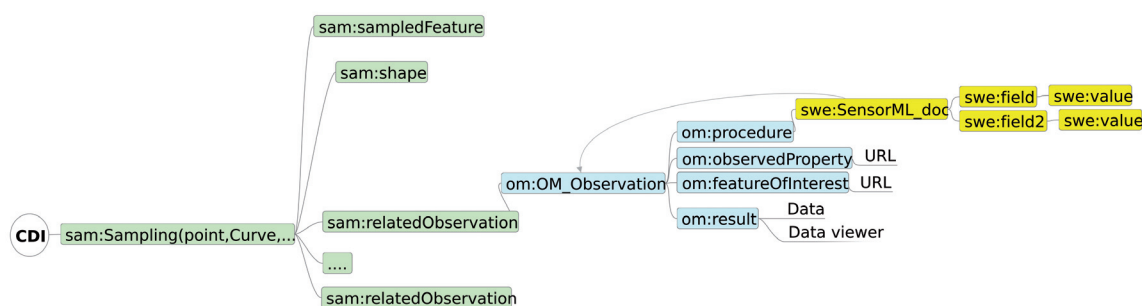
Fig. 1 - GeoSeas metadata model updated and tuned for the needs of SeaDataNet.
