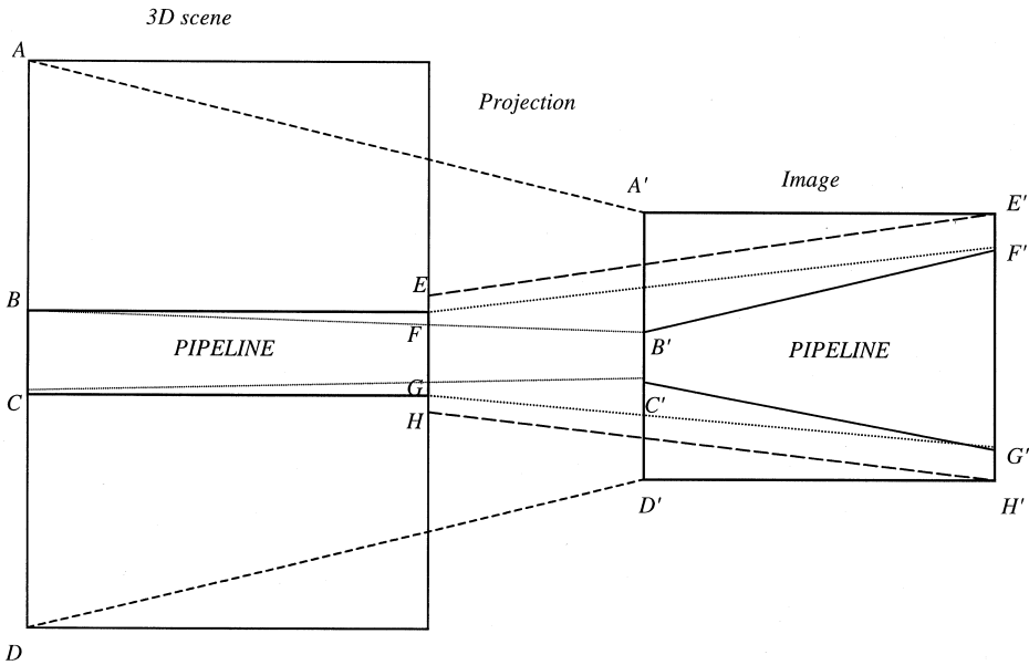
Fig. 7. Transformation of a 3D scene (on the left, seen from the top) into the 2D image registered by the camera (on the right); points corresponding to the ones of the 3D scene are reported on the projection with the apex.
