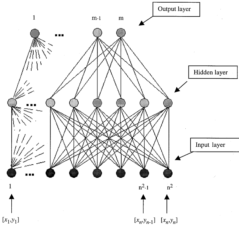
Fig. 3. General scheme of a two layer applied BP model with n^2 input neurons, n^2 hidden neurons and m output neurons. The n \times n subimages to classify are transformed into n^2 vectors and supplied as input to the neural net. The net classifies those images as belonging to one of the m output classes.
