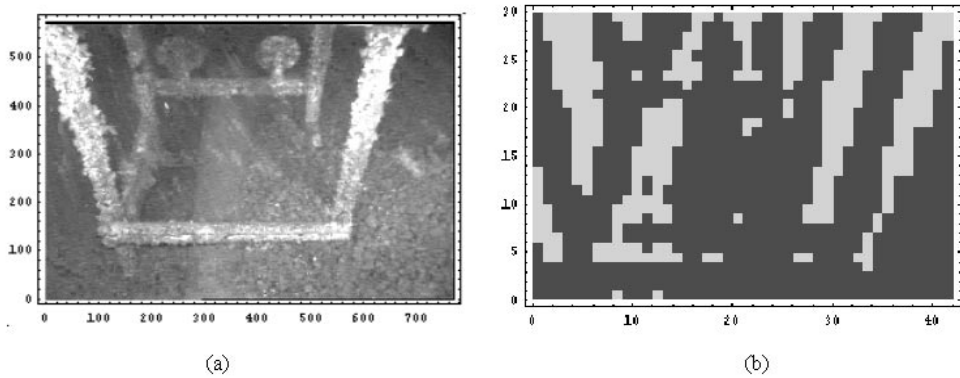
Fig. 11. (a) An example of a trestle object, (b) edge detection by applying neural network to the image in Fig. 7(a).
