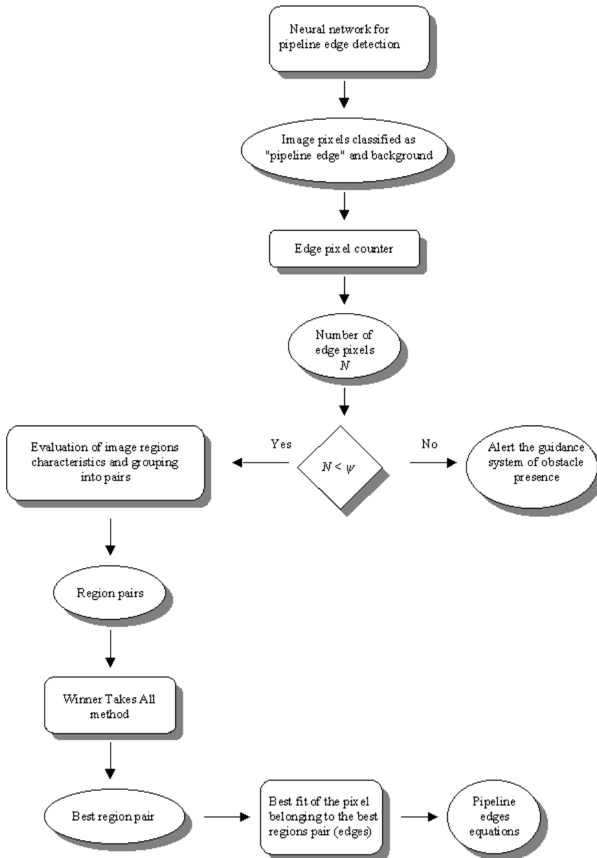
Fig. 2. Edge Detection Module: the module gets as input the image compensated reduced to 1/16 and returns pipeline edge equations in original image reference system.
