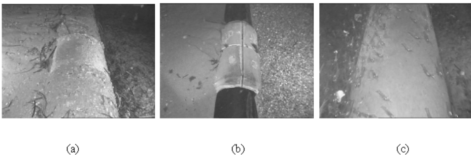
Fig. 12. (a) An anode on a pipeline covered by gunite . There is a small difference of intensity from the anode and the pipeline itself and no difference between the anode radius and the pipeline radius. (b) The gunite is not covering the pipeline. The intensity difference is greater than in the previous case and there is a difference between the pipeline and the anode radius. (c) The AUV is approaching the anode and consequently only a part of it can be seen.
