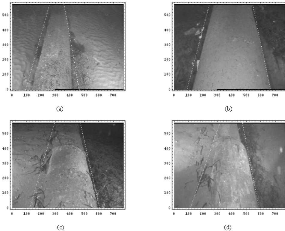
Fig. 14. Some results of the pipeline edge extraction algorithm in different real situations: (a) pipeline on sand and seaweed, (b) pipeline on seaweed, (c) pipeline partially covered by sand, (d) pipeline with a border completely covered by sand.
