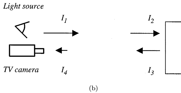
Fig. 5. (a) The main causes of attenuation of the light in water. (b) The original intensity I_1 of the incident wave is reduced near the target to I_2 < I_1 , due to the attenuation of the medium. The reflected wave of intensity I_3 < I_2 , passing again through the medium, is attenuated, and reaches the camera with intensity I_4 < I_3 .
