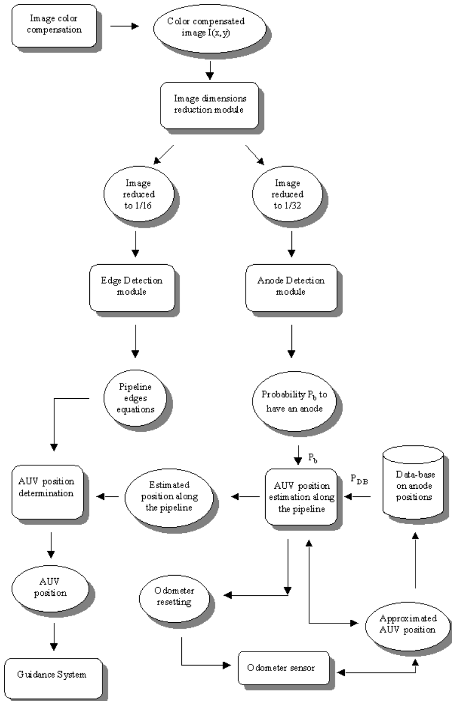
Fig. 1. General flowchart of the proposed system.
