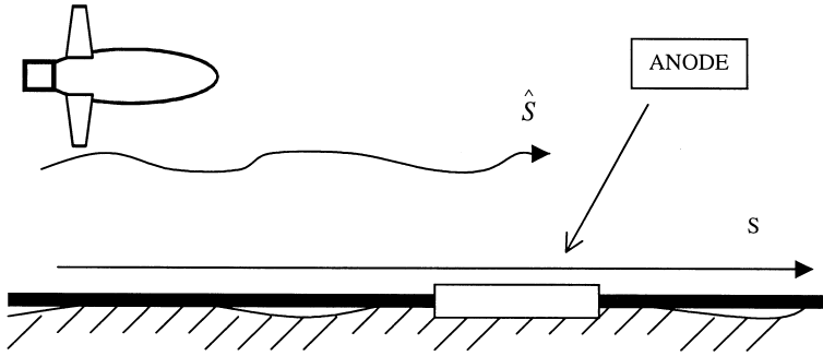
Fig. 13. AUV motion along the pipeline. S is the real coordinate of the AUV and \hat{S} the measured one.
