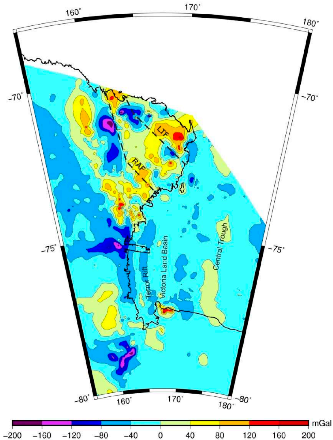
Figure 12. Gridded data of Free-Air Gravity (FAG) anomalies (mGal) in Victoria Land (contour interval at 40 mGal).
