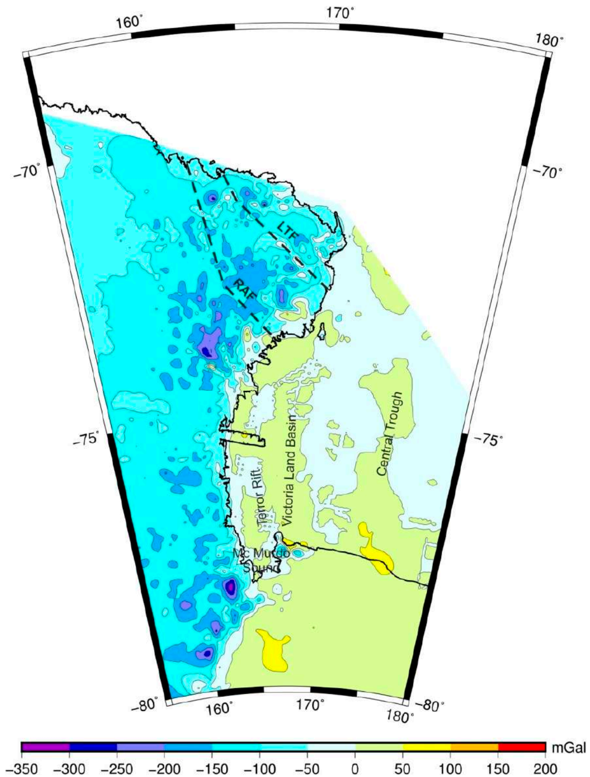
Figure 10. Gridded data of Bouguer Gravity (BG) anomalies (mGal) in Victoria Land (contour interval at 50 mGal).
