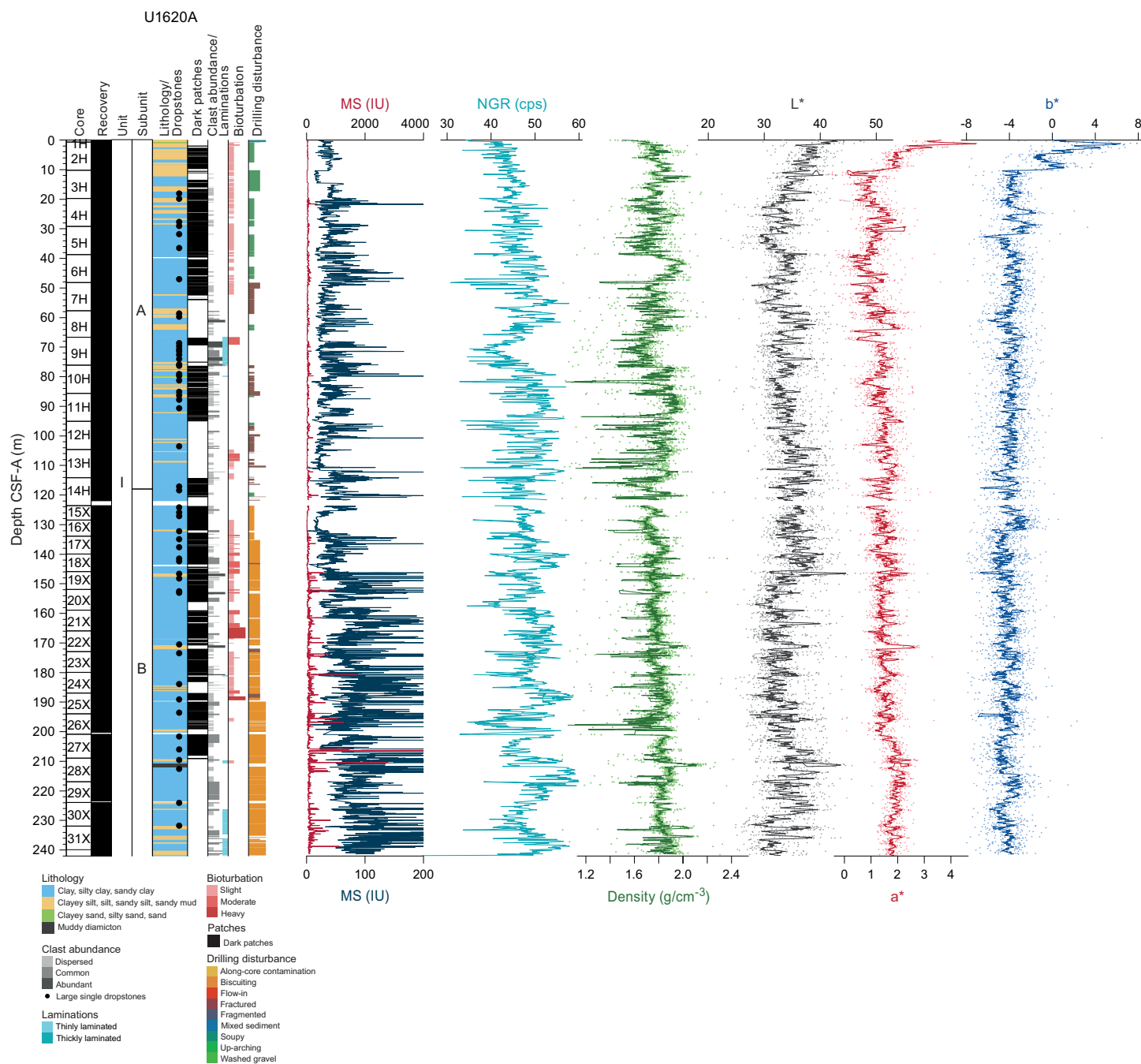
Figure F8. Physical properties, Hole U1620A. Whole-round MS is shown in two different scales, red [0–4000 IU] to display the full range of observed values, highlighting the high values related to greigite/pyrite formation, and blue [0–200 IU] to display the variability of the sediment where greigite is not dominant. Density and CIELAB L^* , a^* , and b^* are displayed as dots superimposed with an 11-point running mean. Unit and subunit boundaries are displayed in relation to their location at section breaks and within core sections rather than at the corresponding depth because overlapping sections occurred due to gas expansion and are not correctly displayed on the CSF-A depth scale. cps = counts per second.
