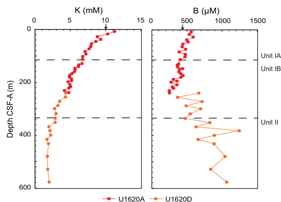
Figure F42. IW potassium and boron, Holes U1620A and U1620D. Black arrows = average seawater values.
