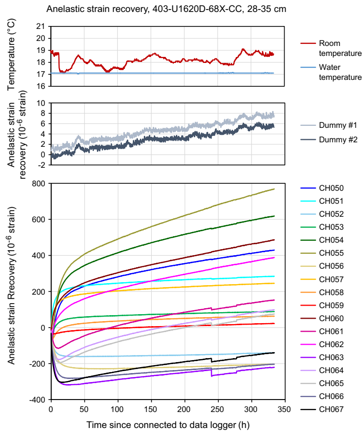
Figure F34. ASR initial results (403-U1620D-68X-CC, 28–35 cm). Top: temperature monitoring data used to ensure water bath temperatures were stable. Middle: results from a dummy channel used to ensure that the data logger was operating correctly. Bottom: average values of the 11 ASR measurements collected from the 18 strain gauges every 10 min for ~14 days.
