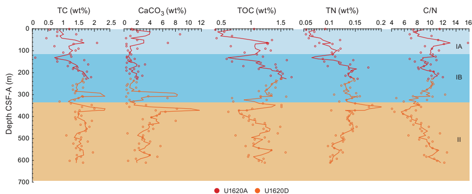
Figure F44. Bulk sediment concentration records with smoothed lines for TC, CaCO 3 , TOC, TN, and C/N ratio, Holes U1620A and U1620D.
