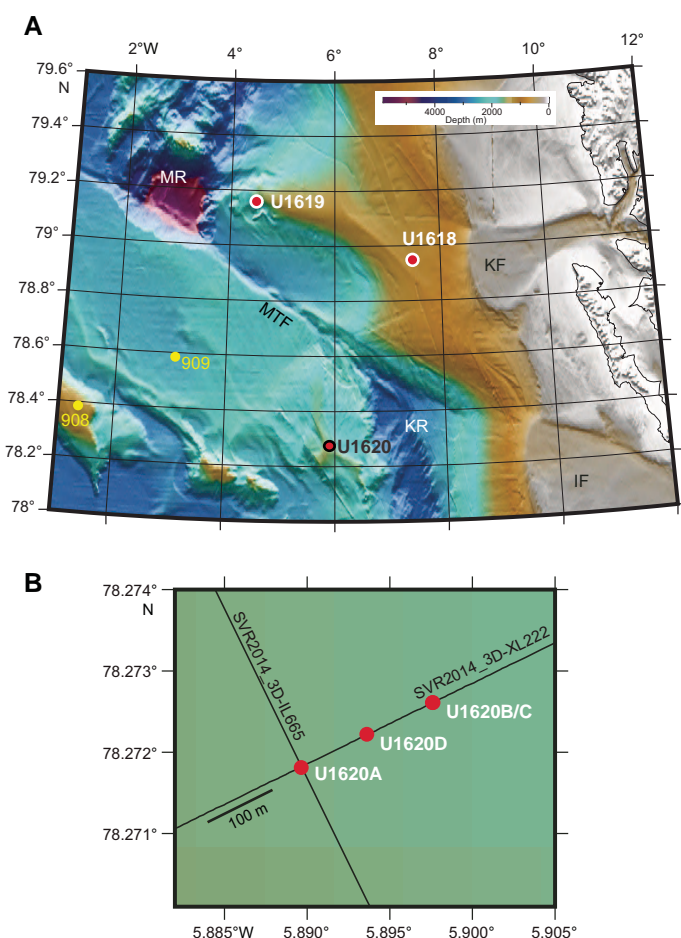
Figure F1. A. Bathymetric map showing the location of Site U1620 on the Svyatogor Ridge sediment drift. Regional bathymetric and tectonic features, locations of the Kongsfjorden (KF) and Isfjorden (IF) glacial troughs and the nearby Expedition 403 and ODP Leg 151 sites are shown. The MTF connects the actively spreading Knipovich Ridge (KR) and Molloy Ridge (MR) segments. Sites U1618 and U1619 are on the eastern and western terminations of the Vestnesa Ridge sediment drift, respectively. ODP Site 909 is on an abyssal hill south of the MTF, and ODP Site 908 is on the Hovgaard Ridge. B. Close-up view of Holes U1620A, U1620C, and U1620D. Hole U1620B (not shown) was abandoned after a poor mudline recovery, and Hole U1620C is located immediately adjacent to it, ~200 m northeast of Hole U1620A. Hole U1620D is located approximately halfway between Holes U1620A and U1620C along Seismic Line Svyatogor2014_3D-XL222.
