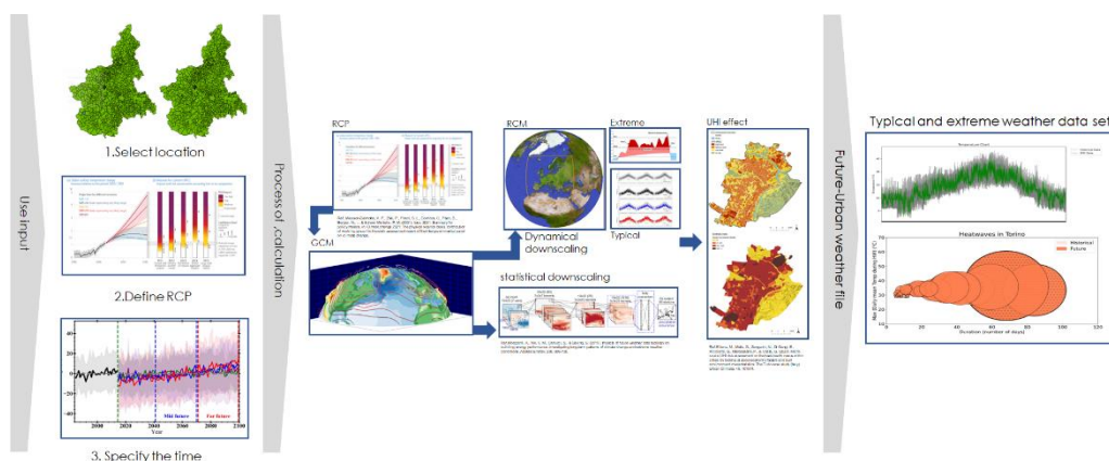
Figure 3 - Process of future weather data.
