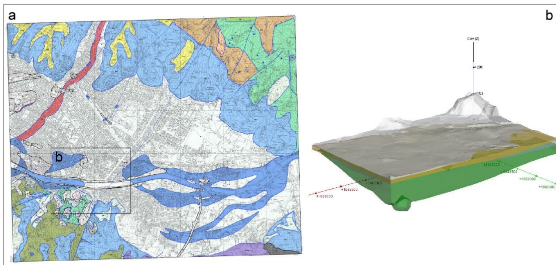
Figure 1. a) The Florence urban settlement as depicted in the 1:10.000 Tuscany geological map (CARG 1:10.000 section n. 275040). The city of Florence well fits with the hypothetical urban settlement proposed in the Scenario n. 5. b) An example of 3D geo-model produced for a portion of the Florence urban area. The 3D model highlights the subsurface stratigraphy and structural setting.
