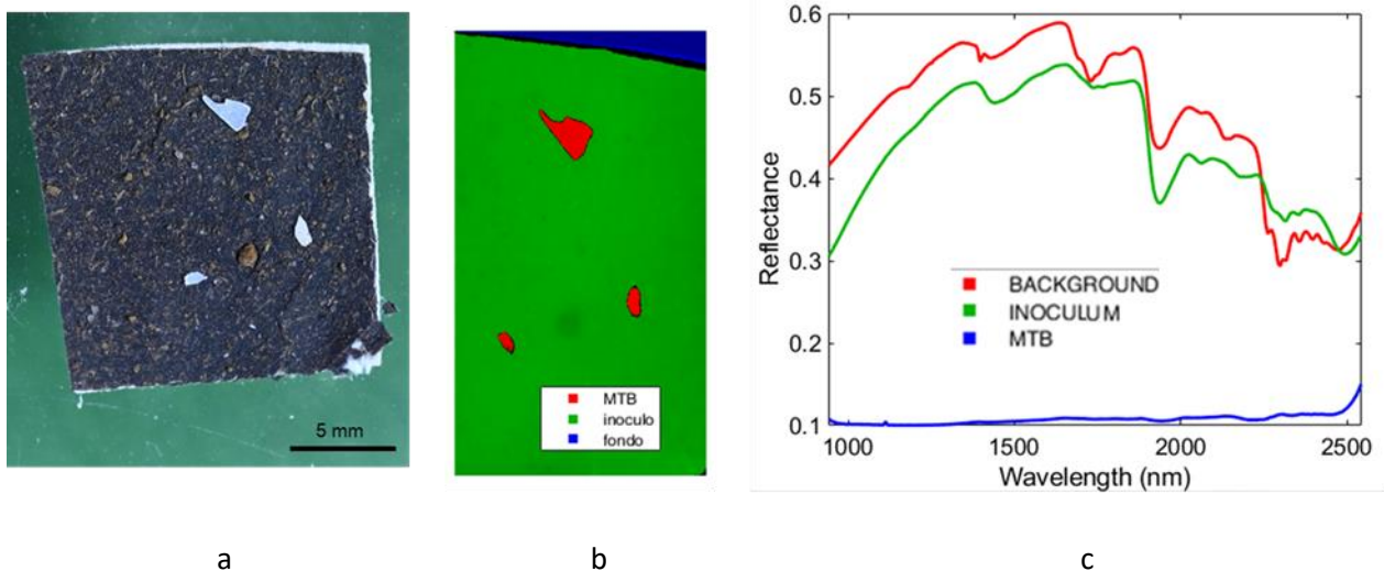
Figure 1 – Mater-Bi® mixed with inoculum, source image (a); false color image with set classes: Mater-Bi® flakes (red), inoculum (green) and background (blue) (b) and average raw reflectance spectra acquired in the SWIR range (1000-2500 nm) of the 3 classes.
