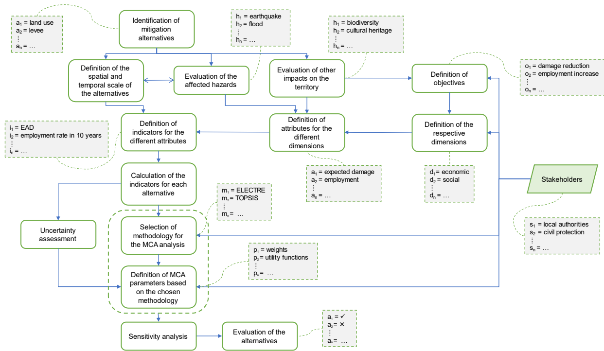
Figure 1 – MCA flowchart.
