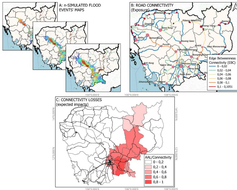
Figure 1 – Connectivity losses with a probabilistic approach. A) n-simulated flood events' maps; B) Road network classified by the edges' connectivity values, and potential origin (red dots)-destination (pink dots, service centers, main cities) pairs; C) Preliminary results showing administrative units classified by the ratio of AAL/total connectivity of road segments in each.
