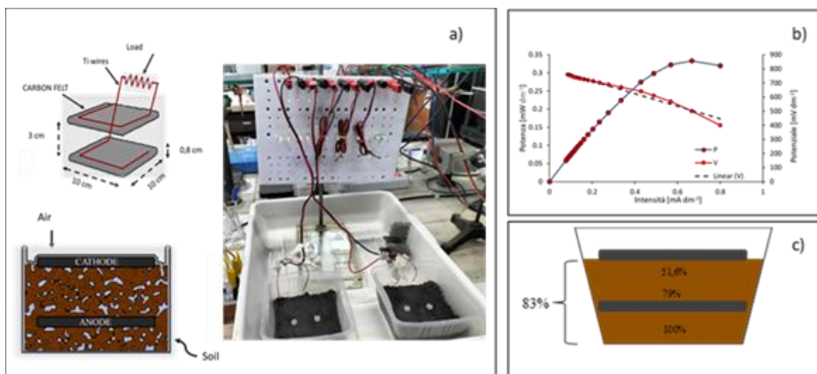
Figure 1 – a) Experimental set-up; b) polarization and power curves of SMFCs; c) percentages of removal of 2,4D in the cell.
