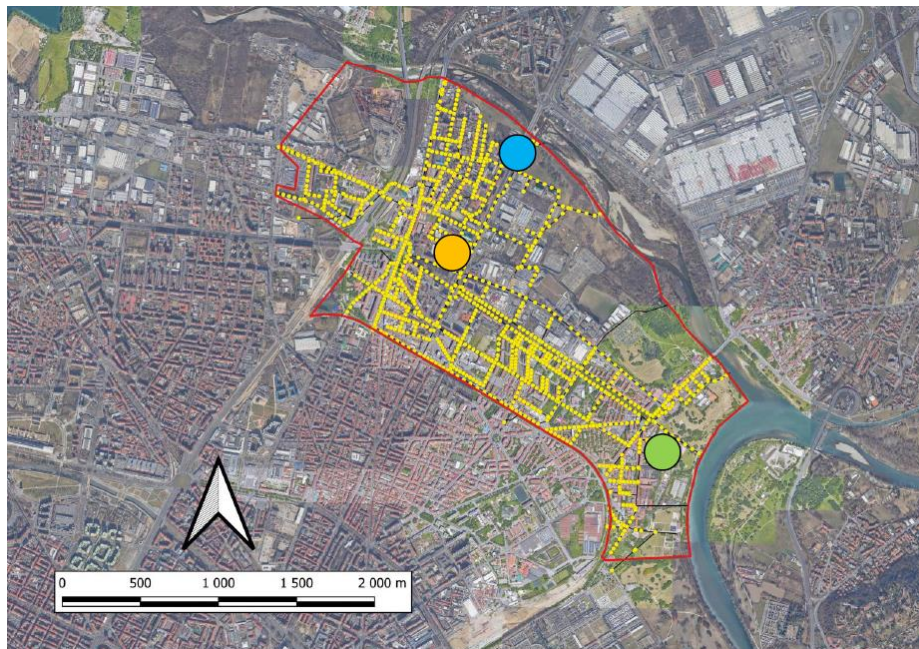
Figure 1 – location of the rain gauges (yellow and green dots) and one flow meter (blue dot).
