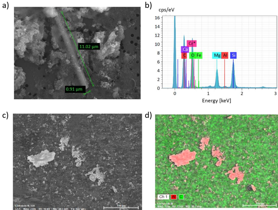
Figure 1 – a) Abbestos fibre acquired using secondary electron detector at SEM, observed in a digested lung biopsy filtered on a polycarbonate membrane. b) EDX spectrum of the abbestosos fibre in (a). c) Aluminum aggregates observed in a digested lymph node biopsy filtered on a polycarbonate membrane. d) EDX mapping highlighting the aluminum (red) and carbon (green) rich areas.
