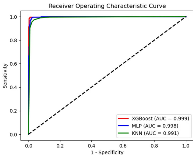
Fig. 8 ROC/AUC plot for ML models
