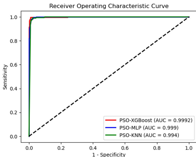
Fig. 9 ROC/AUC plot for PSO-ML models
