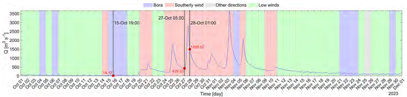
Figure 6. Isonzo River discharge derived from a semi-empirical rating curve based on water level data measurements from the Pieris hydro-metric station. The black vertical lines mark three events: on 15 October at 19:00 UTC with Bora and no outflow, on 27 October at 05:00 UTC with southerly wind and weak outflow and on 28 October at 01:00 UTC with southerly wind and strong outflow. The red dots indicate the values of the discharge rate corresponding to these events.
