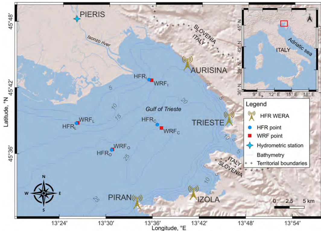
Figure 1. Map of the Gulf of Trieste (size of about 20 × 20 km). Location of HFR network, hydrometric station, points selected in the WRF grid and points selected in the HFR grid in the GoT. The source of the base map is https://server.arcgisonline.com/ArcGIS/rest/services/World_Shaded_Relief/MapServer/tile/{z}/{y}/{x} (last access: 20 March 2025).
